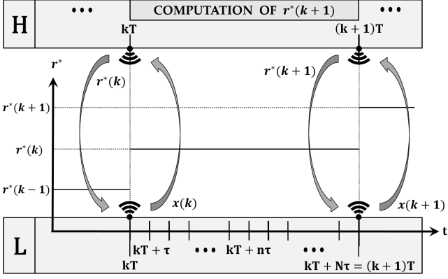
Figure 1. The adopted hierarchical control on two levels and the corresponding time scales
