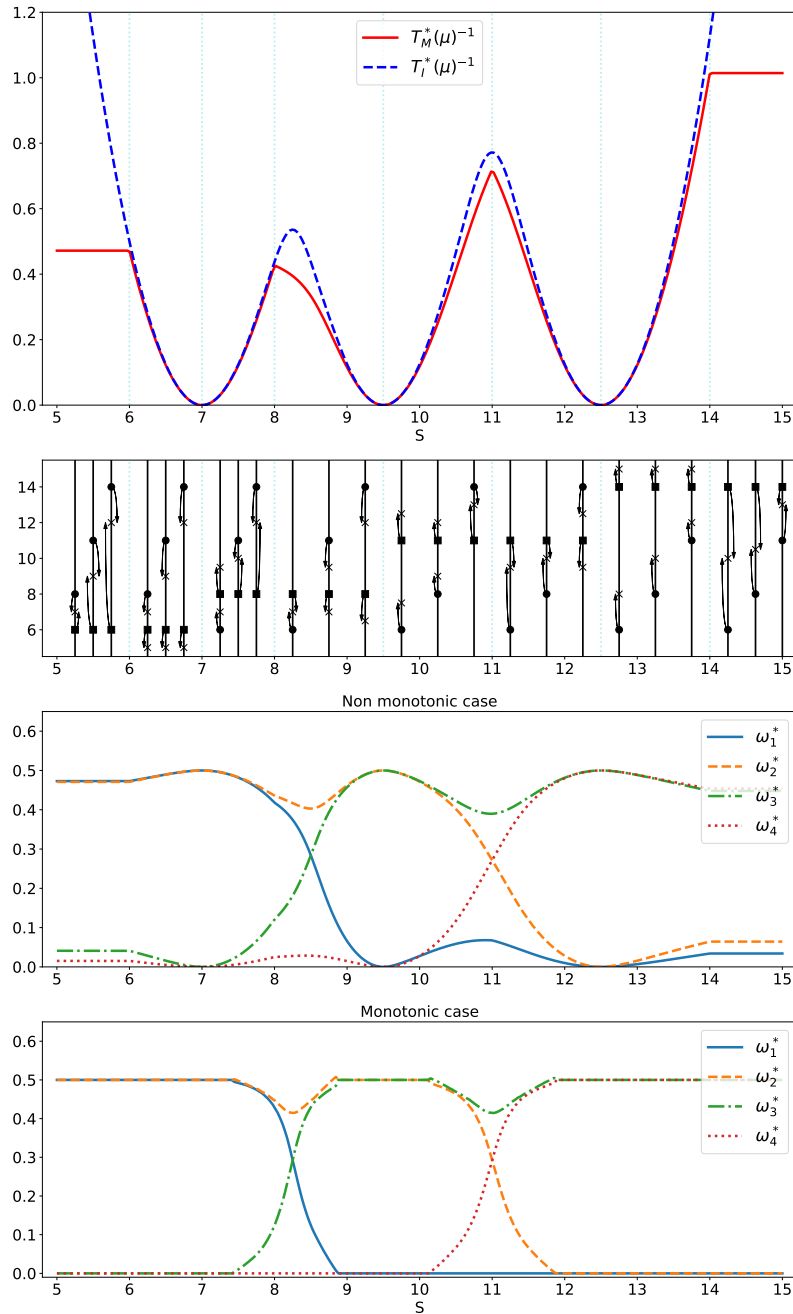
Figure 1: The complexity terms in the bandit model \boldsymbol{\mu} = (6, 8, 11, 14) . Top : inverse of the characteristic time as a function of the threshold S ; red solid line: non-monotonic case \mathcal{S} = \mathcal{M} ; blue dotted line: increasing case \mathcal{S} = \mathcal{I} . Middle : how to move the means to get from the initial bandit model to the optimal alternative in \mathcal{M} . Bottom : the optimal weights in function of the threshold S .
