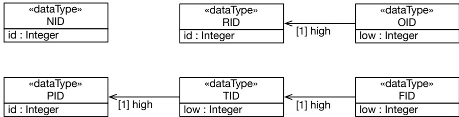
Figure 3: Identity Datatypes
