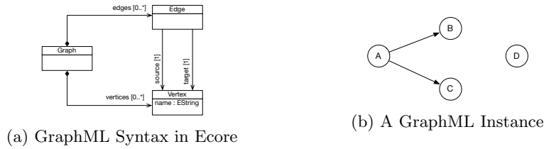
Figure 1: Simple Example
