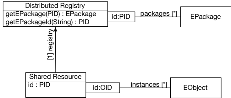
Figure 2: Distributed Registry
