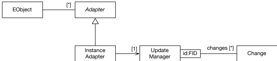
Figure 4: Update Notification
