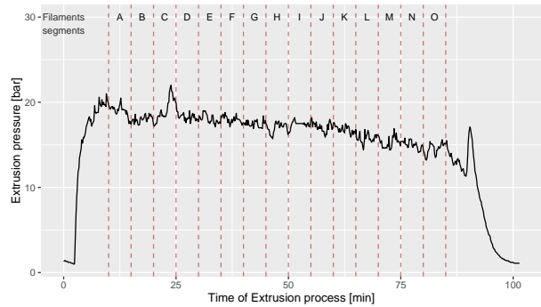
(b) Nozzle pressure in the extrusion process.
