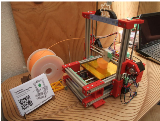
(a) 3D printer -FoldaRap-
