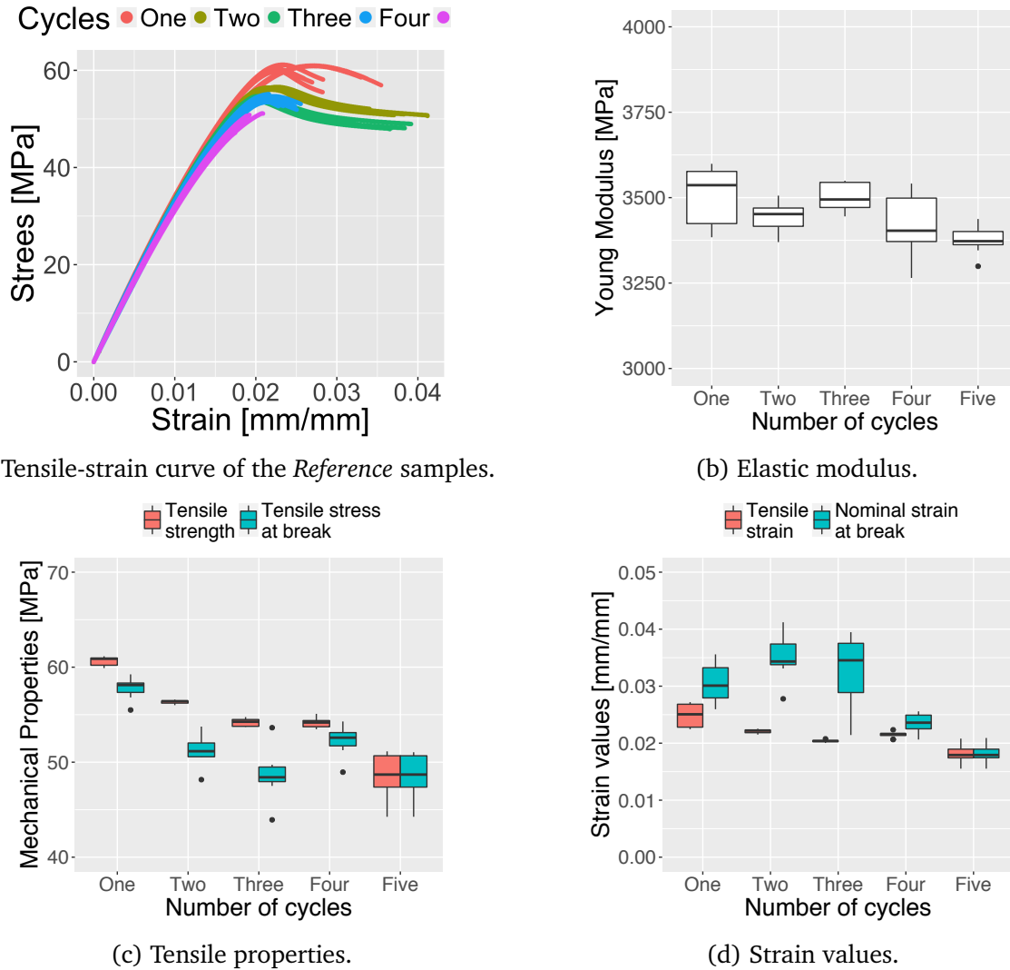
Figure 10: Mechanical properties of the Reference process chain samples
