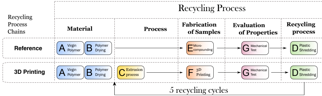
(a) Methodologies for comparing the material degradation using a standard and 3D Printing process.
