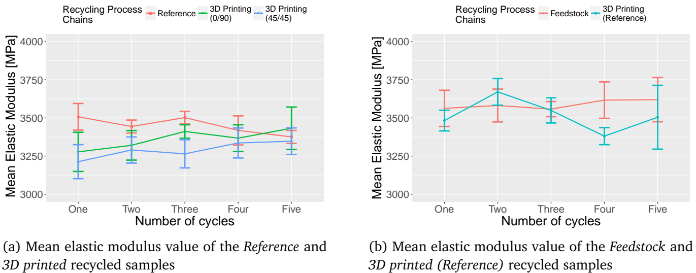
Figure 12: Evolution of elastic modulus in the recycling process chains
