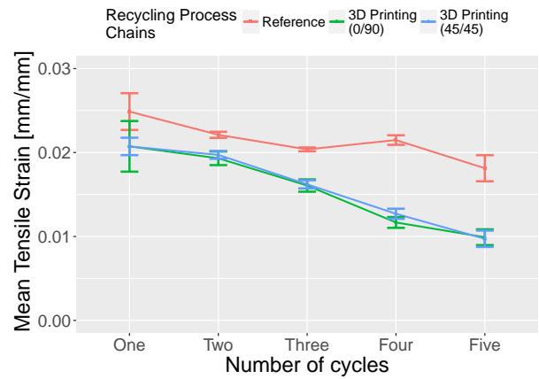
(b) Mean tensile strain values of the Reference and 3D printed recycled samples.
