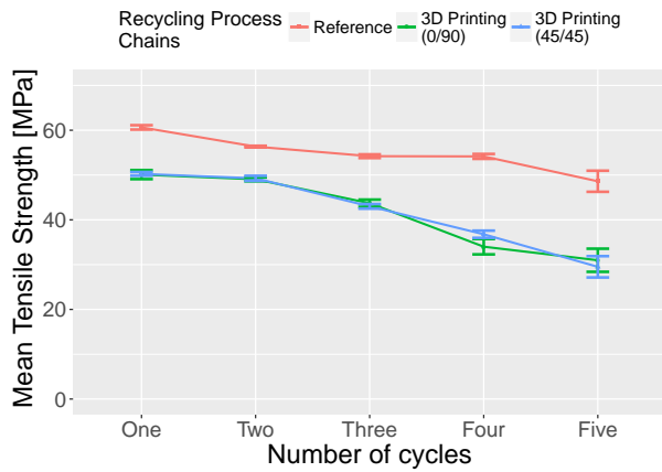
(a) Mean tensile strength values of the Reference and 3D printed recycled samples.
