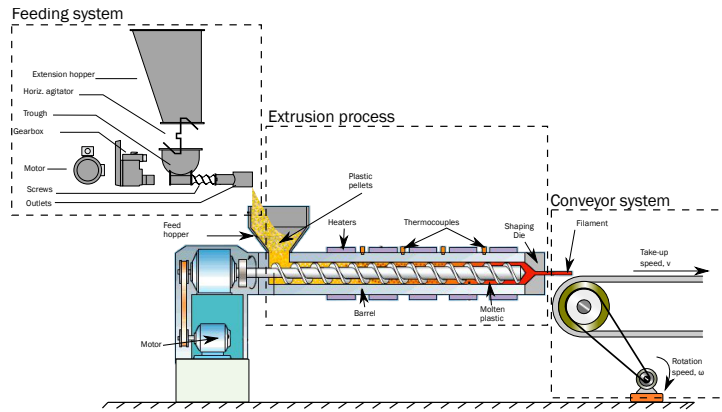
Figure 5: Schematic diagram of the extrusion process for the fabrication of 3D printing feedstock.
