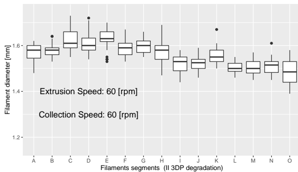
(c) Diameters of the recycled filament segments
