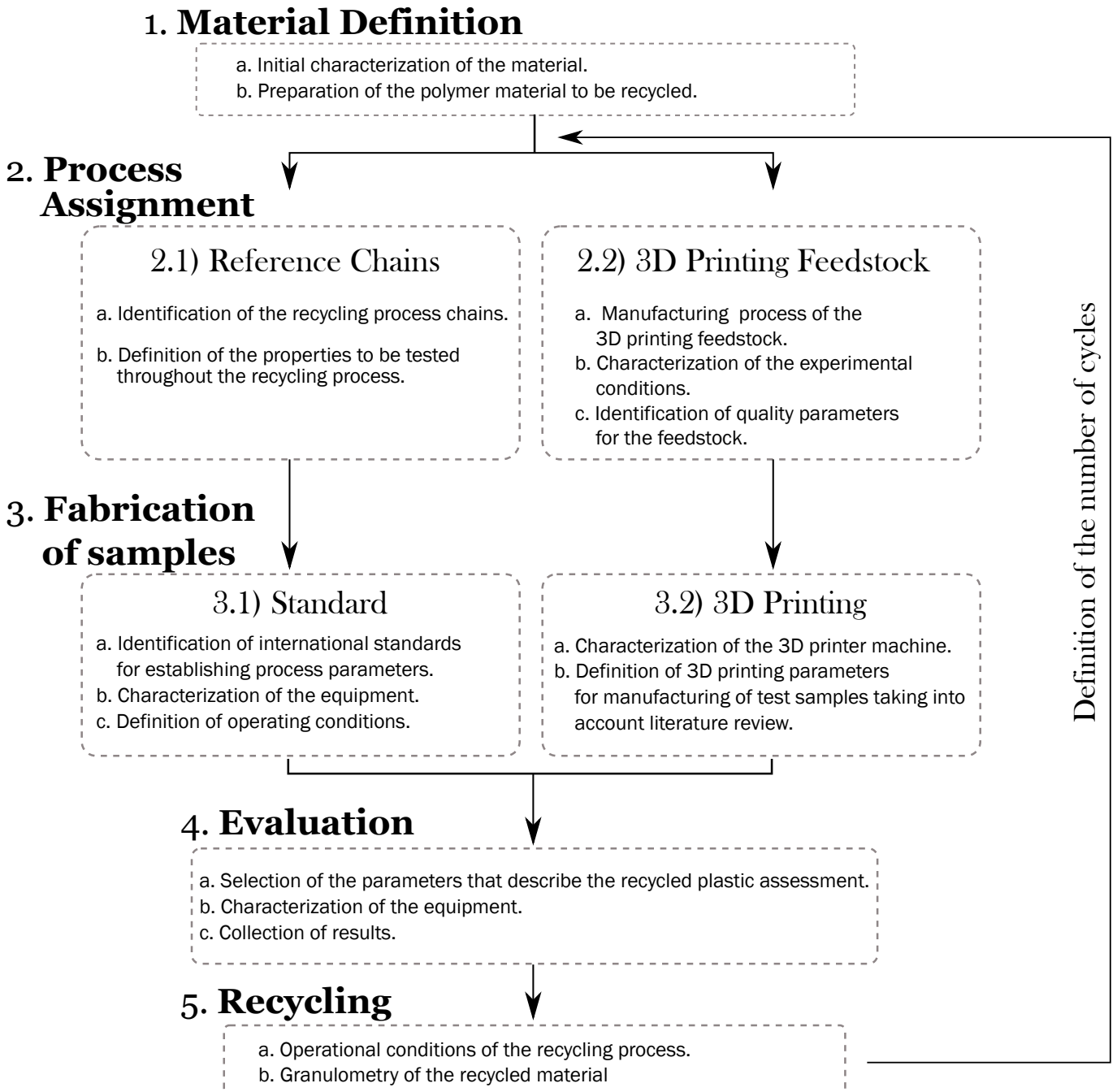
Figure 3: Proposed methodology to evaluate the recycling process in the 3D printing chain.
