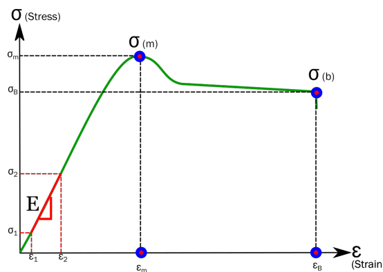
Figure 8: Stress-strain curve.
