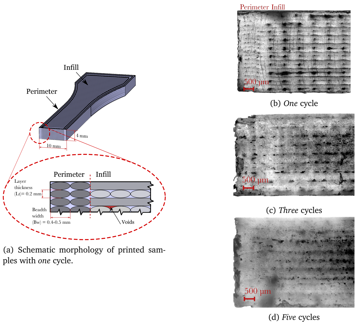
Figure 13: Optical microscopy images for recycled samples (toolpath=0/90) from the 3D printing process chain
