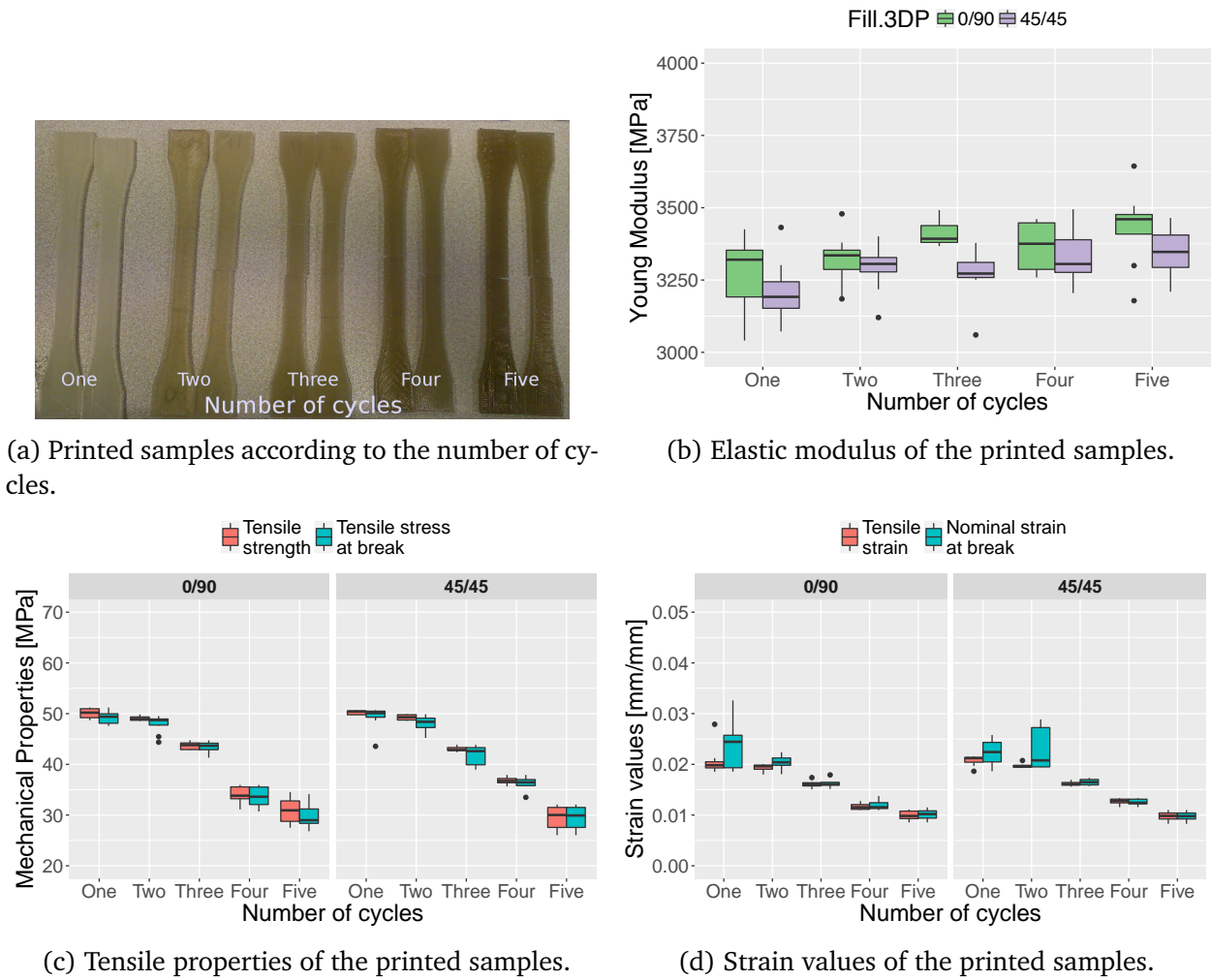
Figure 11: Mechanical properties of the 3D printing process chain samples (0/90 - 45/45).
