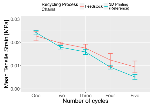
(d) Mean tensile strain values of the Feedstock and 3D printed (Reference) recycled samples.
