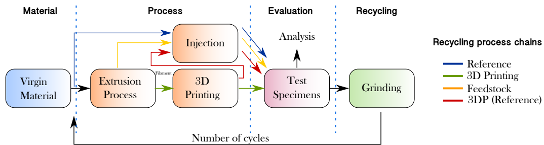
Figure 4: Definition of the recycling process chains.
