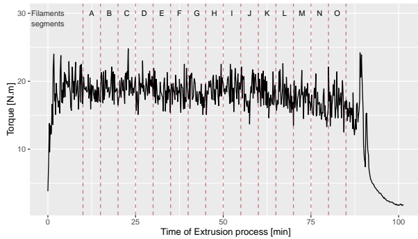
(a) Torque in the extrusion process.
