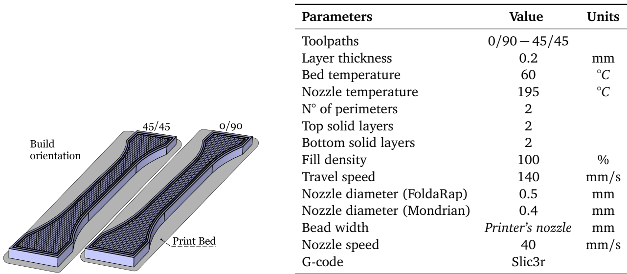
Figure 7: Parameters used for the fabrication of printed mechanical samples
