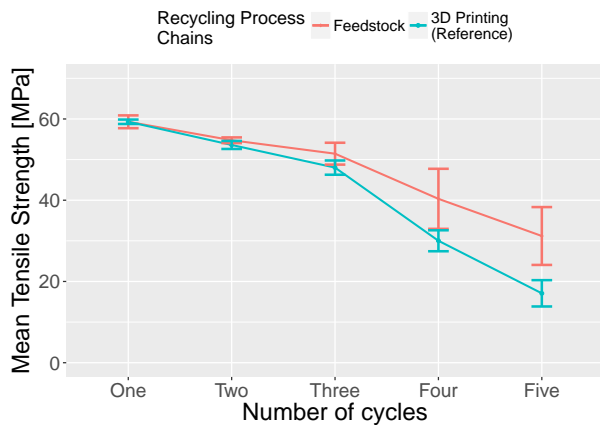
(c) Mean tensile strength values of the Feedstock and 3D printed (Reference) recycled samples.
