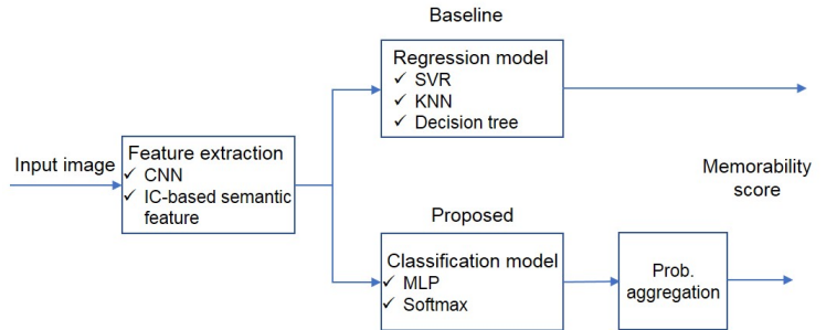
Fig. 1: Workflow of the investigated computational models for image memorability prediction.
