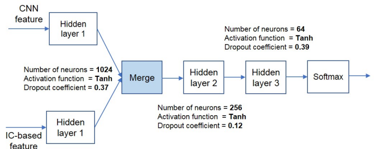
Fig. 2: Best predicting model in terms of average Spearman correlation over a 5-fold validation process.
