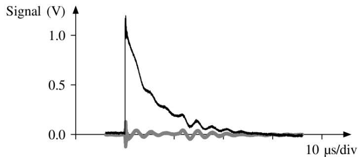
Figure 3. Raw measurements for 50 mA flowing through the gold electrode of a polypropylene material. The laser hits the electrode (black line) or the electrode is masked (gray line).
