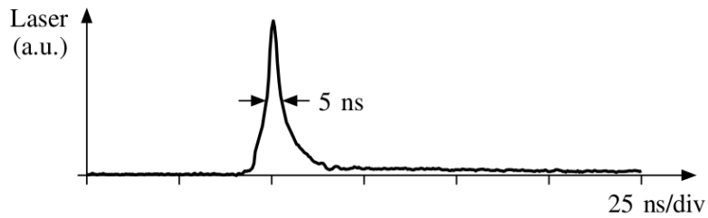
Figure 2. Laser pulse measured by a photo-diode. This is the image of the heat pulse used in thermal measurements.
