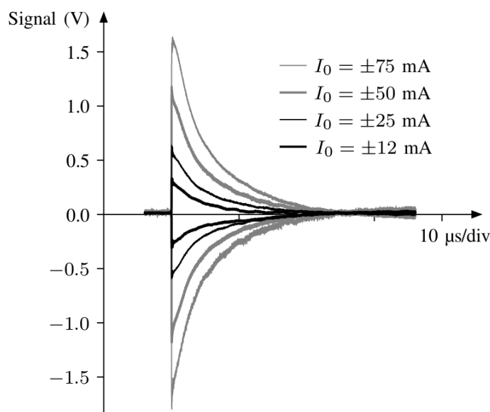
Figure 4. Signals obtained for various currents for the gold-coated polypropylene sample. The dependence of the signal on the current is due to the bolometric effect.
