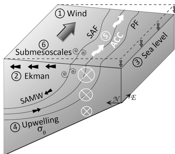
FIG. 1. Schematic of wind-driven upwelling in the Southern Ocean. The ACC, SAF, PF, and SAMW locations are labeled.
