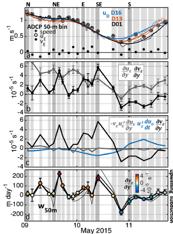
FIG. 8. (a) Time series of alongfront drifter velocity u^D ( \text{m s}^{-1} ) for the three drifters released and followed during the Seasoar survey from 9 to 12 May 2015. Alongfront x and cross-front y water velocity components, u_E and v_E , measured within 1 km of the frontal center are shown for the drifter drogue depth of 50 m. Water speed (*) is also included. (b) Cross-front gradients of u_E (gray) and v_E (black) at 50-m depth and averaged \pm 1 km across the front. Negative \partial \bar{v}_E / \partial y (black) indicates confluent flow. Error bars indicate uncertainty of the ADCP measurements. (c) Estimation of terms in Eq. (9) after making steady-state assumption. (d) Vertical velocity at the drogue depth of 50 m, w_{50\text{m}} ( \text{m day}^{-1} ), with \partial \bar{v}_E / \partial y ( \text{s}^{-1} ), from (b) shown in color. Error velocities of the ADCP are propagated through the calculation of w and are shown as error bars. Additional estimates of w are included for the slab (black) and linear (gray) extrapolations of u_E and v_E to the surface. Vertical velocities and \partial \bar{v}_E / \partial y < 0 indicate subduction and confluence, respectively. The duration of Seasoar legs is shaded in each panel.
