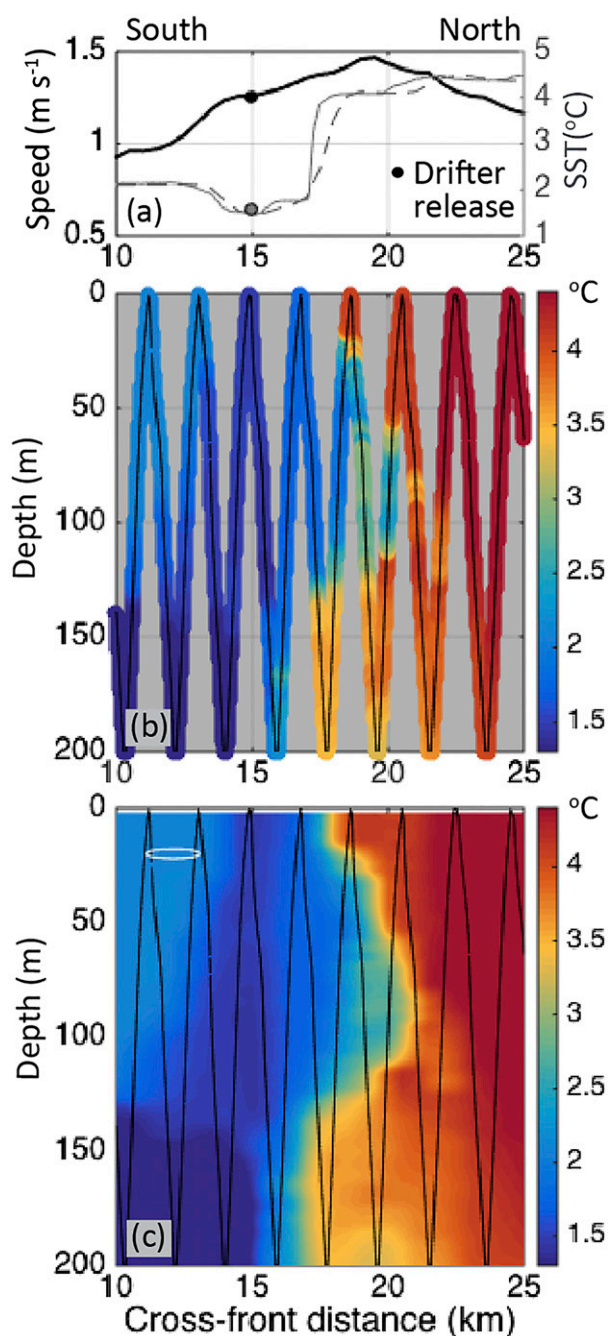
FIG. 3. (a) Measured jet speed ( \text{m s}^{-1} ) at 50-m depth and underway SST ( ^{\circ}\text{C} ) at 4-m depth during the first Seasoar leg in survey. Gridded Seasoar temperature at 5-m depth is dashed. Drifters were released in the cold filament ( 1.56^{\circ}\text{C} ) with jet speed \sim 1.25 \text{ m s}^{-1} , approximately 15 km from the start of the Seasoar leg. (b) Temperature data binned into 0.5-m intervals for the first Seasoar leg. (c) As in (b), but for gridded temperature data with the interpolation window 2 \text{ km} \times 4 \text{ m} shown as an ellipse (white). The location of Seasoar measurements in (b) and (c) are black.
