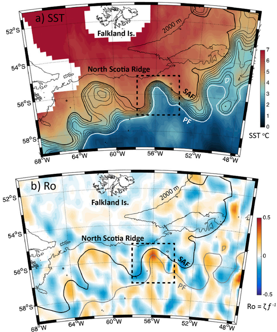
FIG. 2. (a) A northward meander (dashed box) of the ACC in the Scotia Sea, observed remotely on 20 April 2015, is characterized by sharp horizontal gradients of SST ( ^{\circ}\text{C} ; color) and SSH (m; contours). (b) As in (a), but for vorticity Rossby number (color) calculated from altimetry-derived geostrophic surface currents. SSH contours corresponding to the SAF ( -0.25 m) and PF ( -0.70 m) fronts define the northern and southern edges of the meander, respectively. The 2000-m isobath from the General Bathymetric Chart of the Oceans dataset outlines the North Scotia Ridge, the northern boundary of the Scotia Sea.
