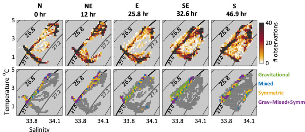
FIG. 10. (a) T - S diagram histograms for Seasoar legs N, NE, E, SE, and S, where color indicates number of measurements in 0.15^{\circ}\text{C} and 0.015 salinity bins and (b) instability types in the mixed layer as diagnosed in section 3d. The cold, fresh observations inside the meander and eddy occupy the bottom-left “hot spot” of measurements in T - S space in leg N. An exchange along isopycnals \sigma_{\theta 27} (thick) and \sigma_{\theta 27.2} (gray) occurs over this series.
