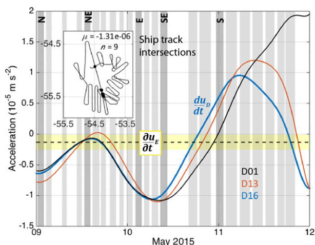
FIG. A2. Estimates of Eulerian local acceleration during the Seasoar survey calculated from ship track intersections (map inset) during the Seasoar survey. Gray bars show the duration of each Seasoar leg; the N, NE, E, SE, and S legs (dark gray) are labeled.
