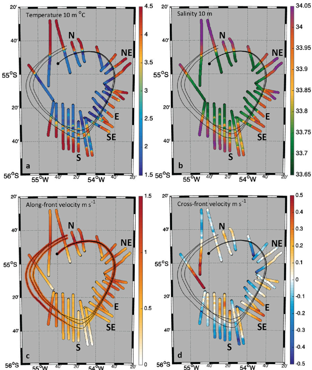
FIG. 5. Maps of 10-m depth (a) temperature and (b) salinity and 50-m depth (c) alongfront and (d) cross-front velocity measurements from the drifter-following Seasoar survey introduced in Fig. 4. A circle marks the starting position of the cyclonic survey. Drifter triplet tracks are shown in black except in (c), where drifter speed is also in color. Positive alongfront velocities indicate a cyclonic (clockwise) direction where positive cross-front velocities indicate flow out of the eddy. Labeled Seasoar legs, indicating the approximate location in the survey, are presented in Fig. 7.
