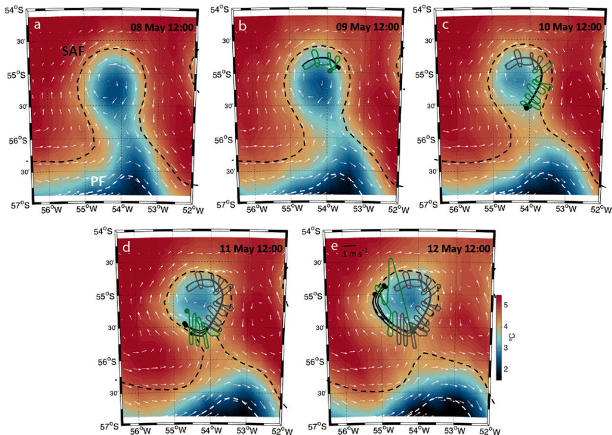
FIG. 4. Daily snapshots of microwave SST (REMSS) and altimetric geostrophic surface current vectors (AVISO) for 8–12 May 2015 capturing the formation of a mesoscale eddy from a northward meander along the ACC in the Scotia Sea (Fig. 2). A drifter triplet (black) was released on 8 May at 2000 UTC in the northwestern sector of the meander and followed while towing the Seasoar with the RRS JCR (green). Positions of the SAF and PF, defined by the -0.25\text{-m} and -0.70\text{-m} SSH contours, are shown in black and white dashed lines, respectively.
