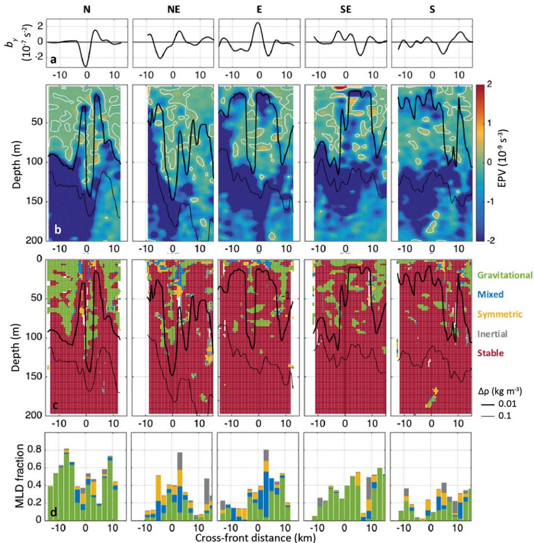
FIG. 9. (a) Cross-front buoyancy gradient b_y ( \text{s}^{-2} ) calculated at 10-m water depth for Seasoar legs N, NE, E, SE, and S. Legs are oriented with the inside of the meander and eddy on the left-hand side of each panel. (b) A two-dimensional estimate of Ertel potential vorticity ( \text{s}^{-3} ) is shown with the zero contour in white and the MLD, defined as a 0.01 (0.1) \text{kg m}^{-3} density difference from the surface, as a thick (thin) black line. (c) Submesoscale instability analysis results based on the Ri_B criteria. (d) Instances of instabilities identified in (c) shown as a fraction of the 0.01 \text{kg m}^{-3} density difference MLD.
