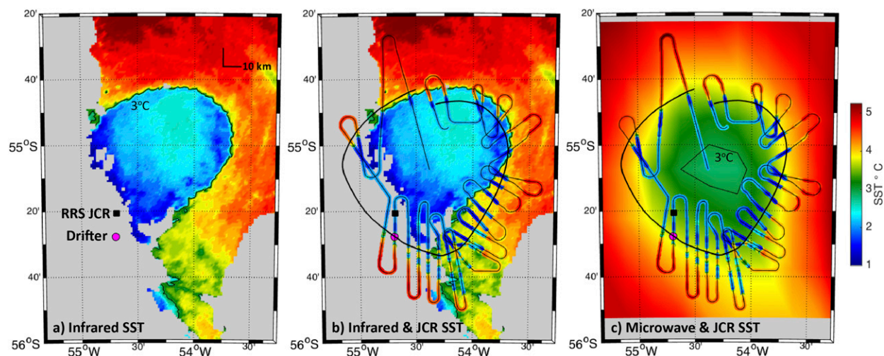
FIG. 6. (a) Level 2 infrared SST measured at 11 May 2015 at 1242 UTC by an AVHRR sensor with 1-km horizontal resolution on the MetOp-A satellite as the drifters (circles) and the RRS JCR (squares) were completing the southwest sector of the Seasoar survey. (b) JCR underway temperature data measured during the survey at 4-m depth and 40-m horizontal resolution overlaid on (a). A drifter track (black) is included. (c) As in (b), but overlaid on microwave SST (OISST; www.remss.com ). The 3°C isotherm (black) outlines the eddy in (a) and the eddy center in (c).
