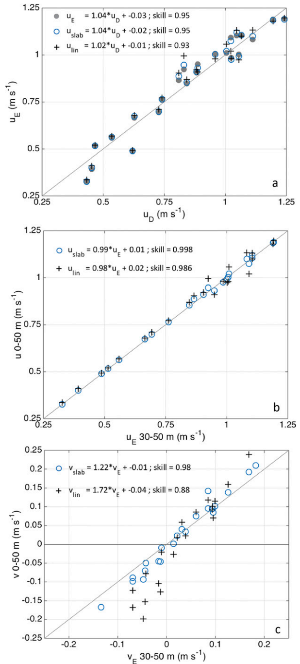
FIG. A1. (a) Drogued drifter velocities ( u_D ) compared with depth-averaged Eulerian velocities between 30 and 50 m ( u_E , ●) and approximations of u_E from 0 to 50 m using slab (○) and linear (+) extrapolations. (b) Comparison of the measured u_E (30–50 m) to the extrapolated approximations (0–50 m). (c) As in (b), but for v_E . Linear regression fits and respective skills, \text{var}(\text{fit})/\text{var}(\text{data}) , are reported in each panel.
