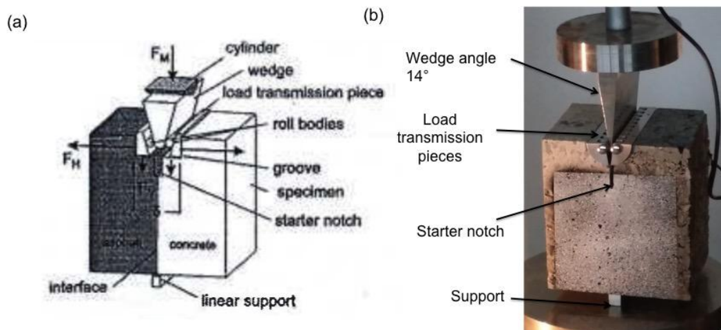
FIG. 1 - The WST test (a) From Tschegg (2007) [9] (b) Adapted by Gharbi et al. (2017a) [10]
