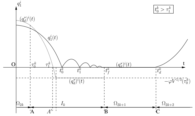
Fig. 2. The design of q_{1d}^* on the transition phases I_k^{J_k}
