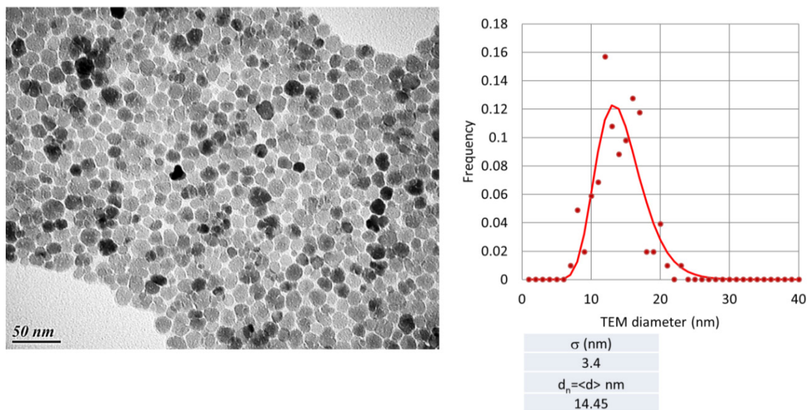
Fig. S1. TEM micrograph and size distribution of moncore IONPs
