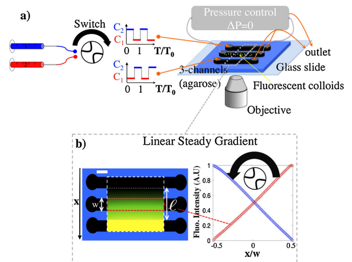
FIG. 1 (color online). (a) Experimental setup (b)-(Left): a 3-channel and gel matrix set-up, superimposed on fluorescence image measured for the stationary gradient of fluorescein with C_1 - C_2 = 10^{-4} M ( w = 300 \mu\text{m} , \ell = 800 \mu\text{m} , scale bar 300 \mu\text{m} ). (b)-(Right): fluorescence intensity profiles measured in stationary state, showing the expected linear profile. Actuation of the microfluidic switch allows us to invert the concentration gradient.
