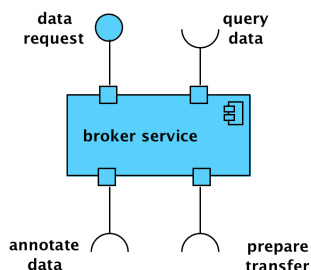
Figure 11: Computational Viewpoint Broker Service object
