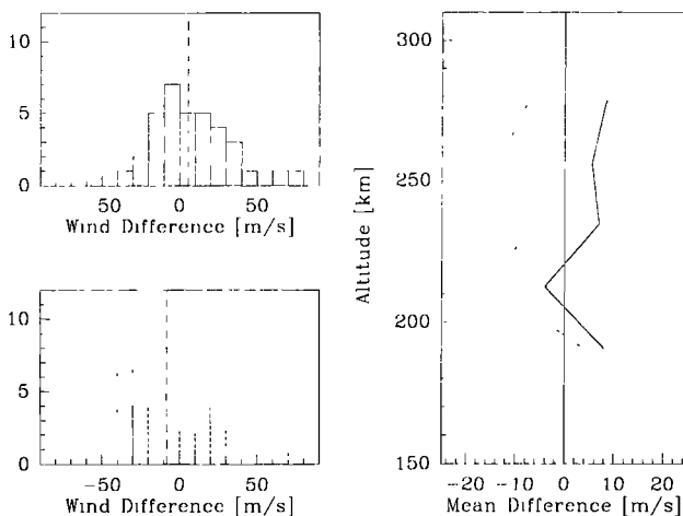
Figure 3. Histograms of (left) the differences between WINDII and EISCAT meridional winds and (right) mean differences as a function of altitude. The upper left panel and the solid line correspond to EISCAT-calculated winds that do not include the Burnside factor. The lower left panel and the dashed line correspond to EISCAT-calculated winds that include the Burnside factor.
