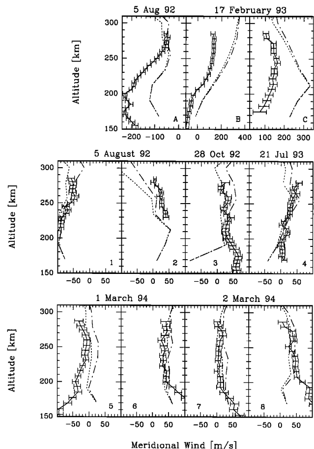
Figure 2. Comparison of the meridional wind profiles measured by WINDII (solid line) and those calculated by EISCAT. The dashed-dotted line is obtained when the Burnside factor is included in the O^+O collision frequency, and the dashed line is obtained when it is not included.
