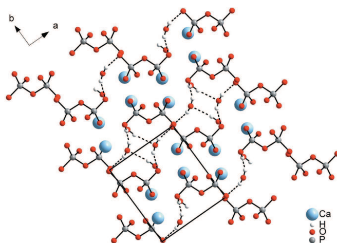
Figure 4 Crystal structure of the t-CPPD phase along the [001] axis showing pyrophosphate anions oriented on (110) and the hydrogen bonding as dashed lines (Mandel, 1975).
