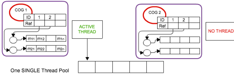
Fig. 6. Thread Creation and Scheduling
