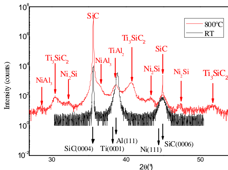
Figure 4. X-ray spectra of Ni/Ti/Al/Ni contacts on 4H-SiC before and annealed at 800°C.
