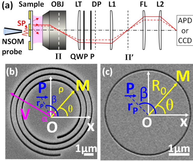
FIG. 1. (a) Sketch of the experimental setup: A linearly polarized laser beam is injected into the NSOM aperture probe or NV-based probe (not shown here). The latter is brought in the near field of the sample to launch SPs. The scattered signal is collected by a microscope objective (OBJ). A removable Fourier lens (FL) enables us to image the back focal plane ( \Pi ). Optical LDOS maps are obtained by raster scanning the sample while maintaining the probe in the near field of the sample. The signal is collected by an optical fiber connected to an APD. Wide-field images of both the direct plane (DP) and back focal plane ( \Pi' ) are captured by a CCD camera. A quarter wave plate (QWP) and polarizer (P) enable circular polarization analysis. Scanning electron microscope images show (a) a spiral and (b) circular plasmonic structure with geometrical parameters used in the theoretical study. Point P represents the position of the tip with \mathbf{r}_p = \mathbf{OP} := [r_p, \beta] and M the position of an electric dipole on the groove described by \mathbf{OM} := [\rho, \theta] for the spiral and \mathbf{OM} := [R_0, \theta] for the circular cavity. The pink arrow represents the vector \mathbf{V} = k_{\text{SP}}\mathbf{r}_p + \rho\mathbf{k} for the spiral cavity defined as \mathbf{V} := [V, \alpha] .
