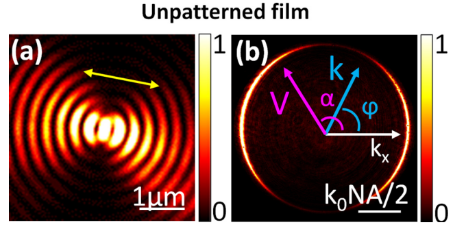
FIG. 2. SP excitation on an unpatterned 50 nm thick gold film by an aperture probe: CCD images of (a) the direct and (b) the Fourier plane. In (a), a beam blocker is placed in the Fourier plane to remove the light directly transmitted through the sample. The yellow arrow indicates the polarization direction of the dipole. In (b) we show geometrical parameters used in the theoretical study: the blue arrow represents the wave vector defined as \mathbf{k} := [k, \varphi] ; the pink arrow represents the vector \mathbf{V} = k_{\text{SP}}\mathbf{r}_p + \rho\mathbf{k} for the spiral cavity defined as \mathbf{V} := [V, \alpha] .
