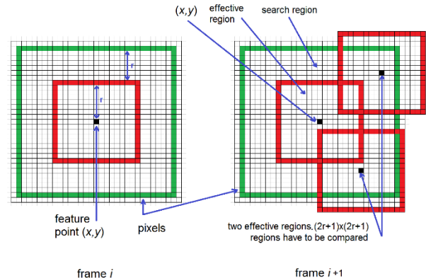
Figure 5: Parallel-pipeline implementation of the proposed feature matching algorithm.
