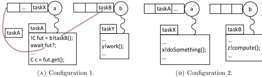
FIGURE 1. Cooperative scheduling in Creol.
