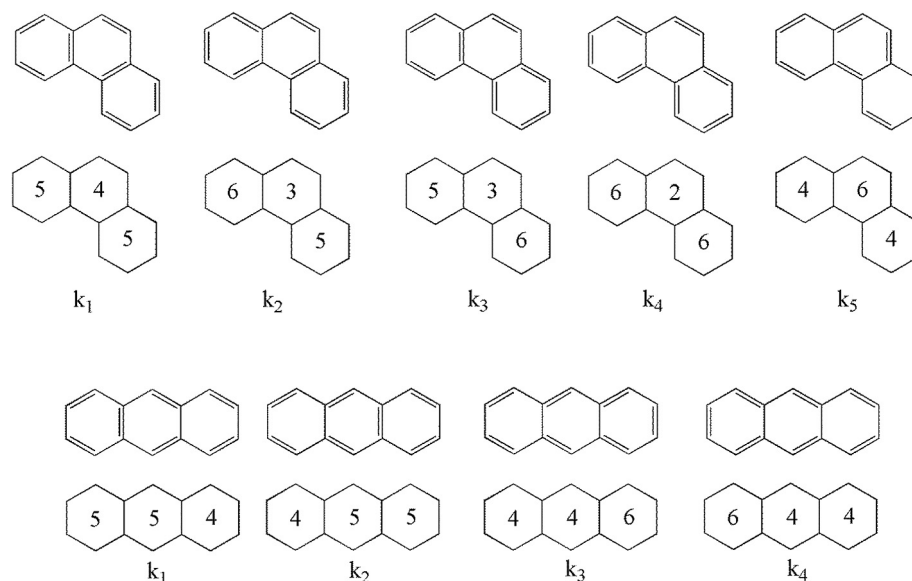
Fig. 1. Kekulé structures and algebraic Kekulé structures of phenanthrene and anthracene.
