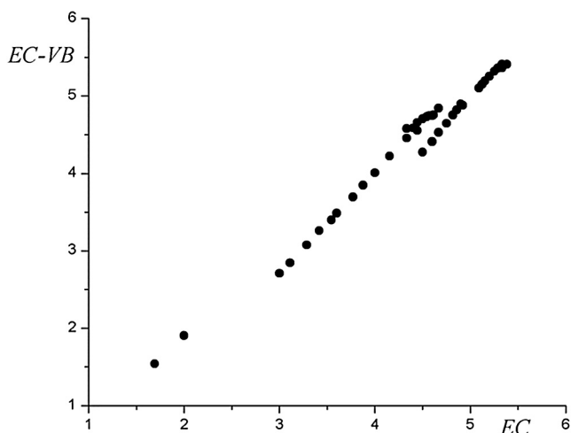
Fig. 3. Correlation between the VB-EC and EC values calculated for the symmetry-nonequivalent rings in the studied benzenoid molecules ( 1–14 ); the correlation coefficient is R = 0.9914 .
