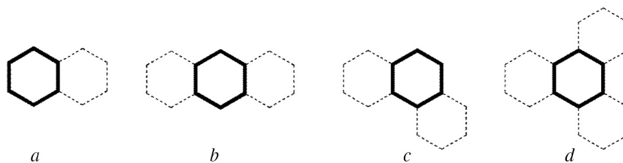
Fig. 6. The four different annelation modes of hexagonal rings that can be found in the studied benzenoid molecules 1–14.
