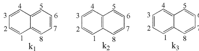
Fig. 7. Kekulé structures of naphthalene and of all its aza derivatives (Fig. 2) and the numbering of the sites in naphthalene where nitrogen atoms can be positioned.
