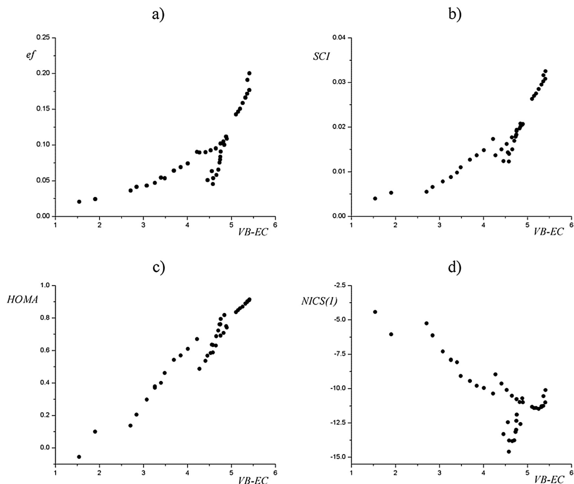
Fig. 4. Dependence of the values of different aromaticity indices for 43 symmetry unique hexagonal rings in molecules 1–14 on the VB-EC values obtained with the STO-6G basis set: (a) ef vs. VB-EC ; (b) SCI vs. VB-EC ; (c) HOMA vs. VB-EC and (d) NICS(1) vs. VB-EC .
