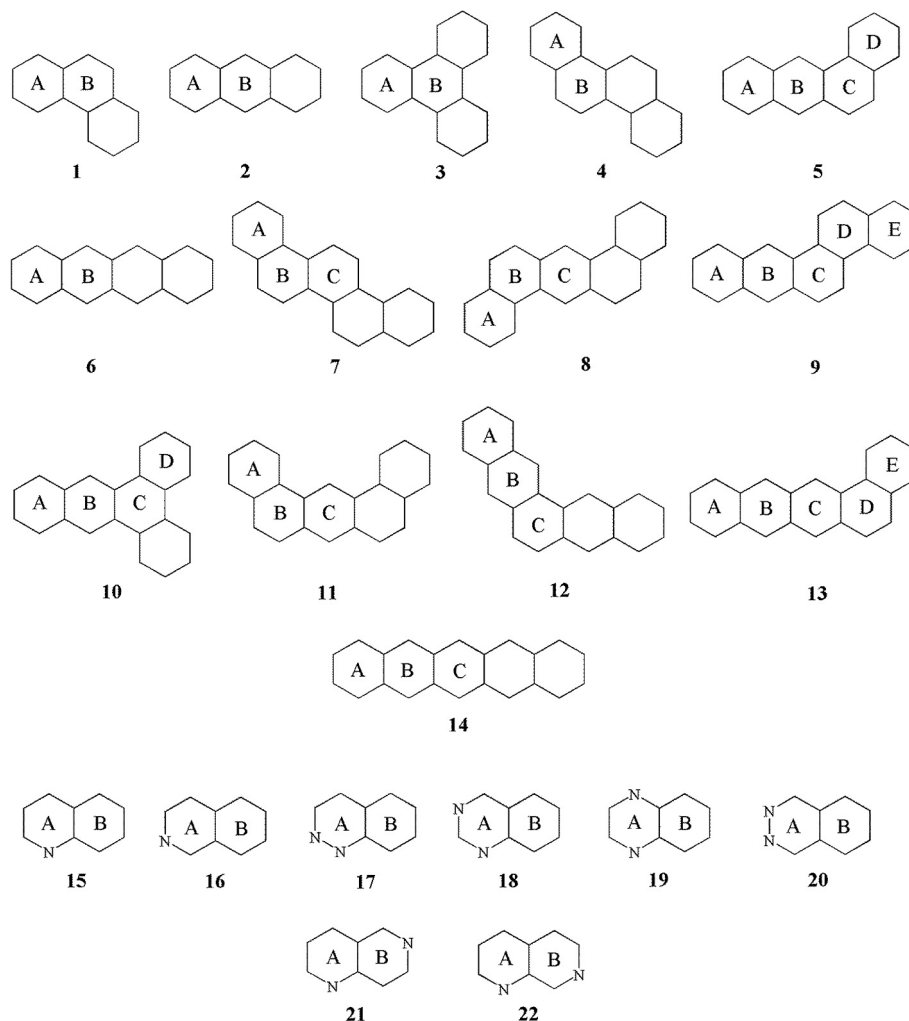
Fig. 2. Set of polycyclic conjugated molecules studied with the molecular nomenclature employed; symmetry unique rings are denoted by capital letters.
