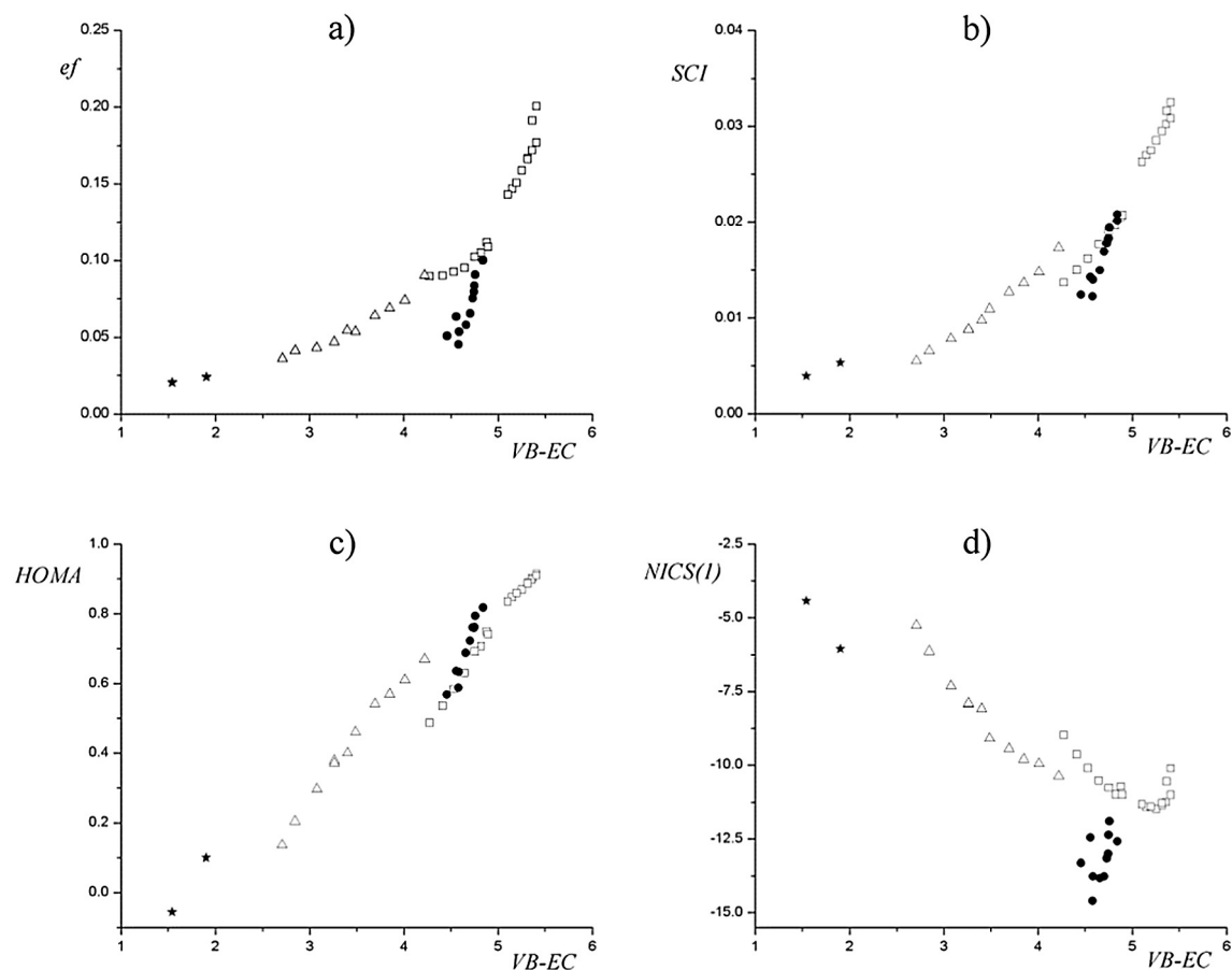
Fig. 5. Same data as in Fig. 4; the data-points are separated into four clusters, pertaining to four annelation modes: mode a (squares), mode b (circles), mode c (triangles), and mode d (asterisks) (cf. Fig. 6).
