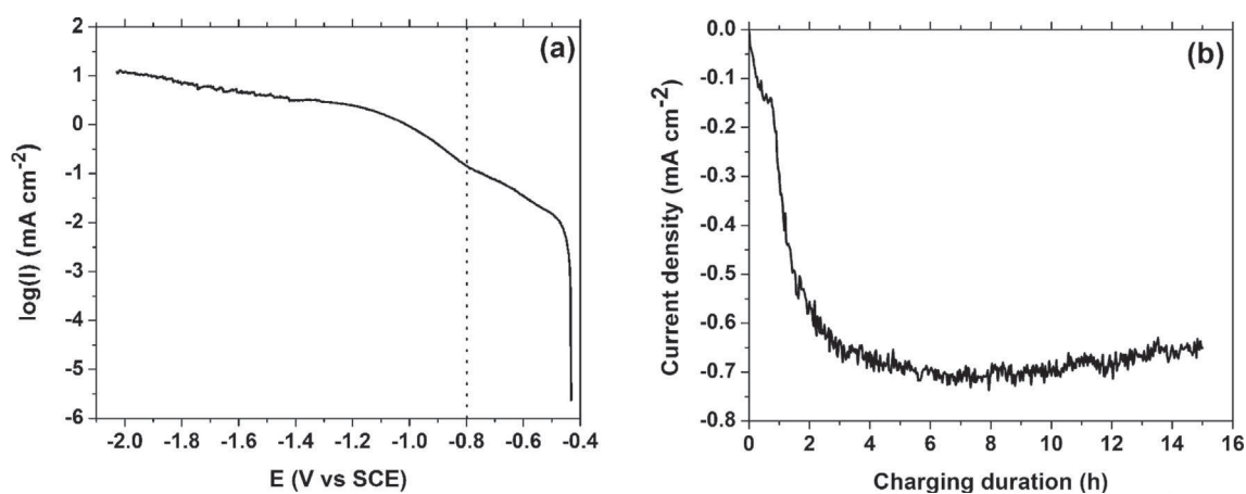
Fig. 1. (a) Polarization curve for AA 2024 in 10 mM H 2 SO 4 at 25 °C. Scan rate = 1 V h -1 . (b) Charging curve at E = -0.8 V/SCE.
