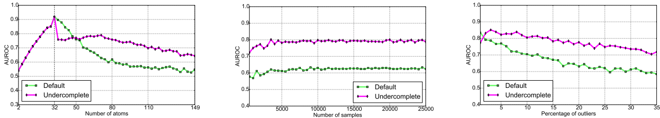
(a) Different dictionary sizes, with 1000 samples and 10% are outliers. (b) Different number of samples, where 10% are outliers. (c) Different outlier ratios (%), with 1000 samples and 64 atoms.
