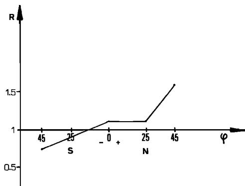
Fig. 10. Ratio R = [O]_{200} December 1969/ [O]_{200} June 1969 for different latitudes.
