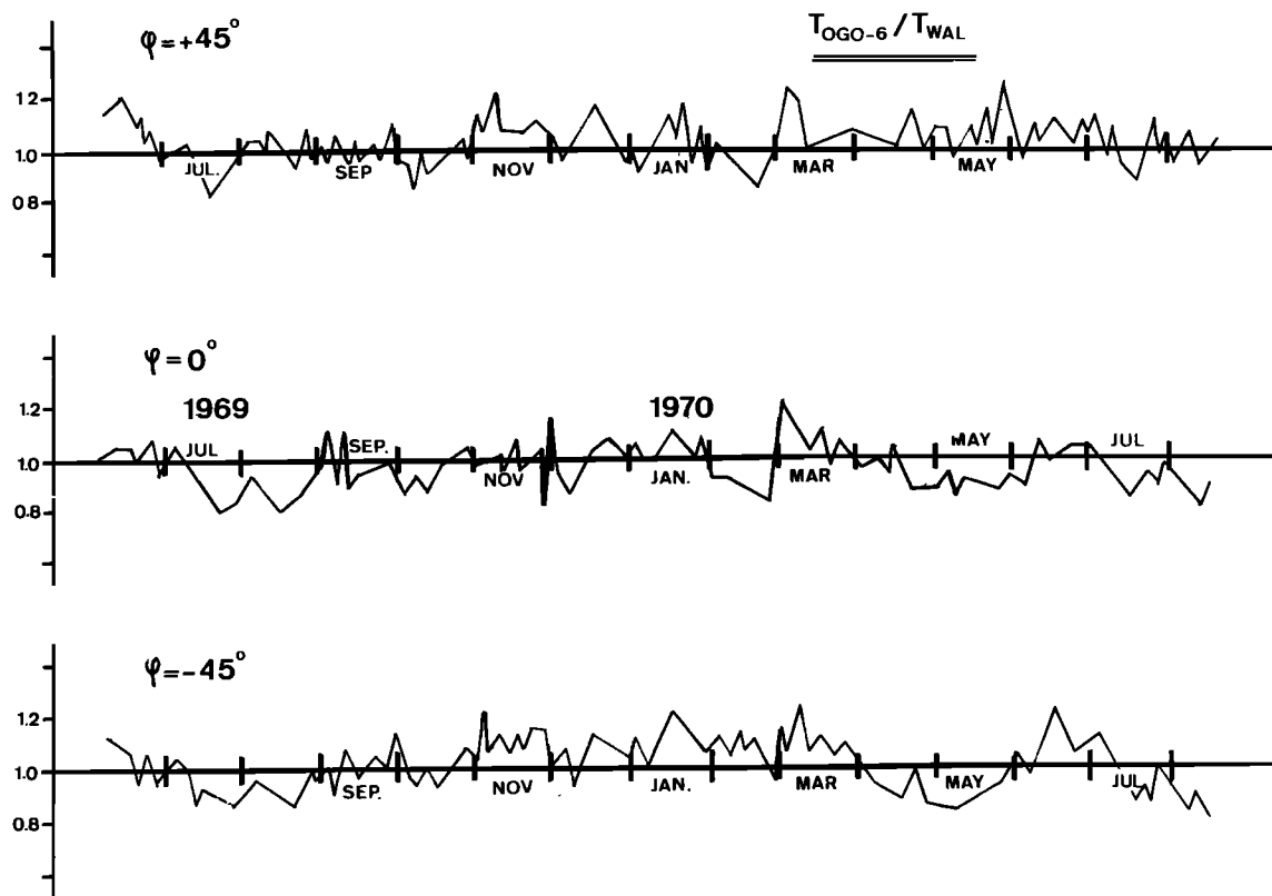
Fig. 3. Ratio of the observed temperatures T_{Ogo\ 6} and the temperatures obtained by using the Waldteufel model, T_{Wal} .
