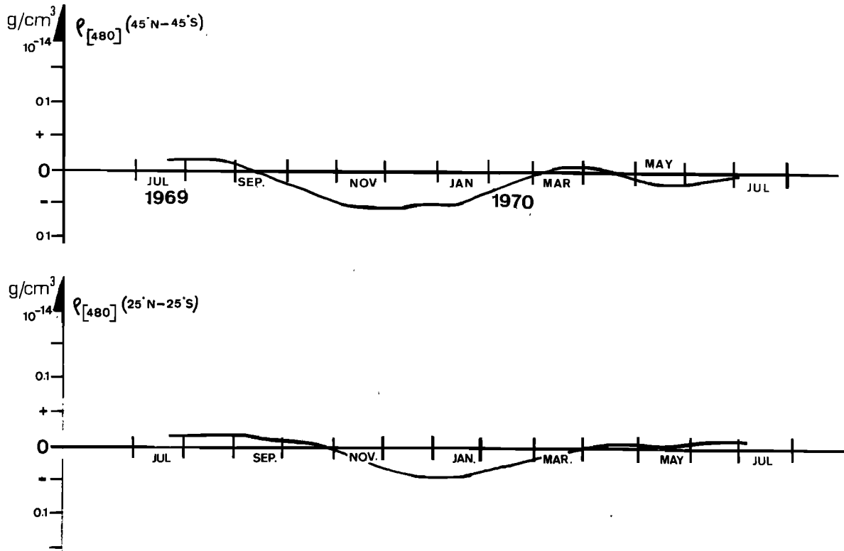
Fig. 8. Difference between northern hemisphere and southern hemisphere densities at 480 km, deduced from statistical analysis, for the same period and geometrical position as the Ogo 6 temperature measurements.
