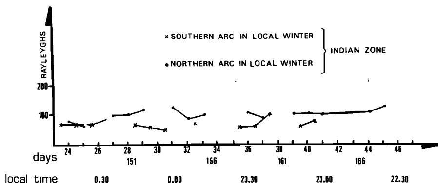
Fig. 11. Comparison of the intensity of the northern arc in December (local winter) with that of the southern arc in June (local winter).
