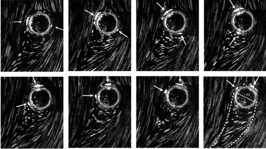
FIGURE 5. ‘Partly contaminated’ surface (DW-1 and DW-2): time interval between two images is 20 ms. The particles stuck on the surface are spinning, Re \approx 50 . The arrows are included to help follow some of these particles. On the last image, the visually estimated edges of the wake are shown by the dashed lines. Sign + designates the rear region of the bubble where particles at the surface have a speed greater than \omega , while sign = corresponds to the front region where the particles have a constant speed \omega .
