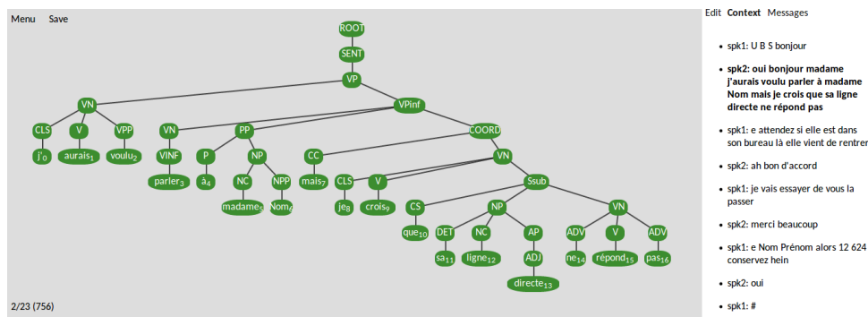
Figure 1: Output of the second phase: Standford parse tree on the pre-processed sentence (1).
