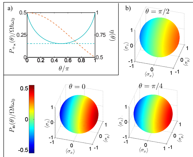
FIG. 2: Performance of the measurement powered engine. a) Orange dotted-dashed line: normalized extracted power P_{+_{\mathbf{x}}}(\theta)/\Omega\hbar\omega_0 ; Solid blue line: MPE yield \eta(\theta) as a function of the Rabi angle \theta ; Dashed blue line: thermally driven engine's yield \eta_{\text{cl}} . We chose \hbar\omega_0/(2k_{\text{B}}T_{\mathcal{D}} \log(2)) = 2 . b) Normalized extracted power P_{\mathbf{n}}(\theta)/\Omega\hbar\omega_0 in the Zeno limit where \theta \rightarrow 0 , as a function of the chosen operating point |+_{\mathbf{n}}\rangle for \theta = \pi/2 , \theta = \pi/4 and in the Zeno limit \theta \rightarrow 0 .
