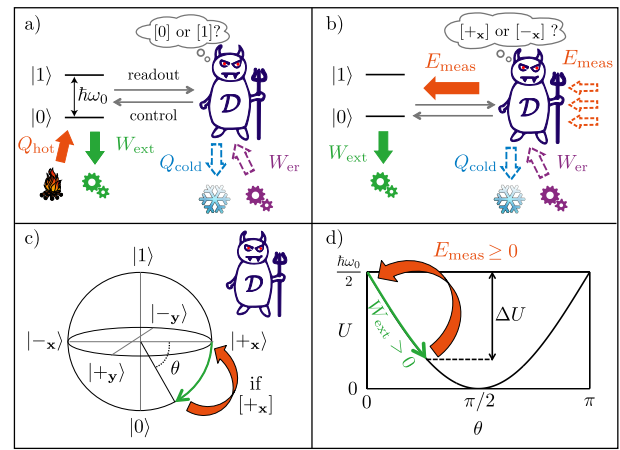
FIG. 1: Maxwell's demon assisted engines. a) Thermally driven engine. The working agent is a qubit of transition frequency \omega_0 . A demon measuring in the qubit energy basis \{|0\rangle; |1\rangle\} allows to convert the heat Q_{\text{hot}} extracted from a bath into work W_{\text{ext}} . The demon's memory is erased by some extra-work source at the minimal work cost W_{\text{er}} while the heat Q_{\text{cold}} is evacuated in a hidden cold bath. b) Measurement Powered Engine. In case the demon measures in the \{|+x\rangle; |-x\rangle\} basis, work can be extracted from the measurement channel and no hot bath is required. c) Evolution of the qubit state in the Bloch sphere. Between two measurements delayed by \tau_w , the evolution induced by the driving field is a rotation around the Y axis at Rabi frequency \Omega (green thin arrow). The measurement projects the qubit on states |\pm x\rangle (orange thick arrow). d) Evolution of the qubit internal energy U(t) = \text{Tr}[\rho(t)H(t)] as a function of the Rabi angle \theta = \Omega\tau_w . During the Hamiltonian evolution the work W_{\text{ext}} = -\Delta U is extracted into the driving field. The measurement provides the energy E_{\text{meas}} = W_{\text{ext}} back to the qubit.
