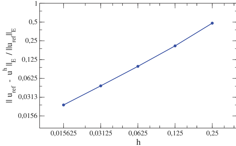
FIG. 3. Relative errors in energy norm for Example 1.
