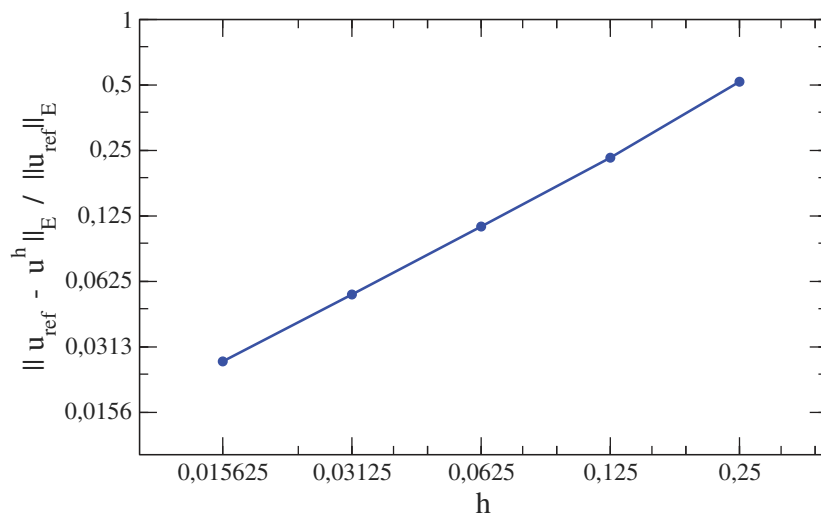
FIG. 6. Relative errors for Example 3.
