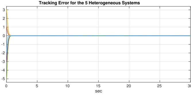
Fig. 2. Tracking error of the 5 followers with respect to the reference trajectory.
