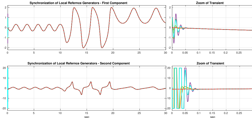
Fig. 1. Synchronization of the local reference generators y_k^{\text{ref}} on the leader's trajectory. The leader's trajectory is plotted as a dashed-dotted red line: during the transient, the local reference generators saturates according to the chosen values and ultimately synchronize on the leader's trajectory.
