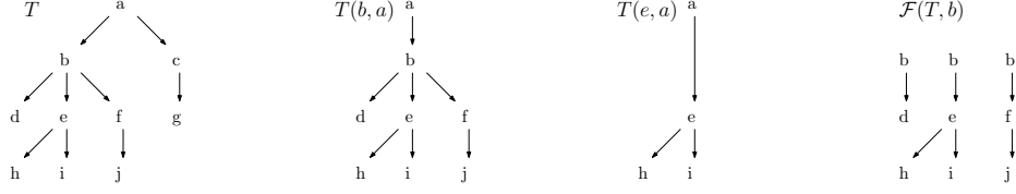
Fig. 2. Examples for a rooted tree T .
