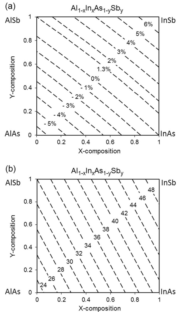
FIG. 4. Curves of (a) iso misfit with InAs substrate and (b) iso average Z versus chemical composition, for quaternary alloys.
