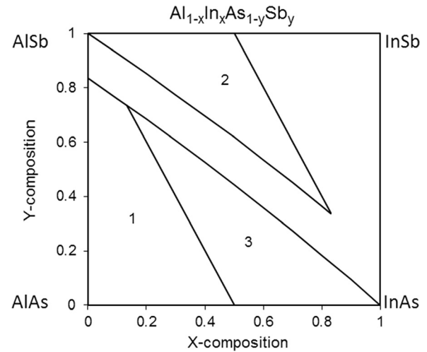
FIG. 7. Quaternary compounds composition from HRTEM and HAADF-STEM analysis.
