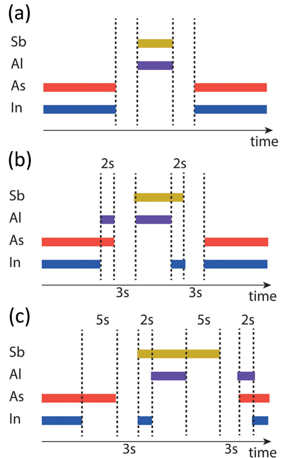
FIG. 1. Growth sequence of the samples. (a) In sample A, the interfaces are spontaneously assembled. (b) In sample B, we tried to make AlAs then InSb interfaces, whereas in sample C (c) we tried to make InSb then AlAs interfaces.
