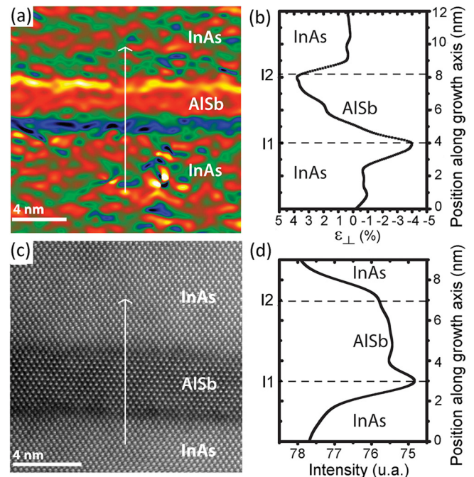
FIG. 8. (a) \varepsilon_{\perp} mapping of sample B, from GPA of a [110] zone axis HRTEM image, (b) \varepsilon_{\perp} strain profile averaged on the whole width of the image (30 nm), (c) HAADF-STEM micrograph of sample B, (d) intensity profile of this HAADF micrograph plotted along the growth direction.
