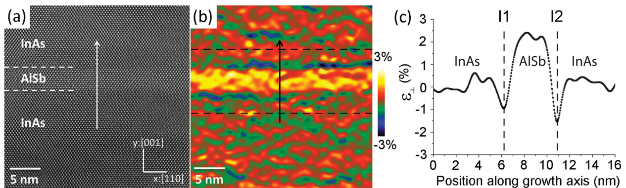
FIG. 5. (a) HRTEM image of sample A along [110] zone axis, (b) \varepsilon_{\perp} mapping, (c) \varepsilon_{\perp} strain profile obtain by GPA averaged on the whole width of the image (30 nm). The white arrow indicates the growth direction.
