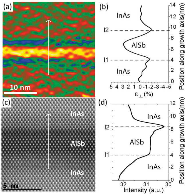
FIG. 9. (a) \varepsilon_{\perp} mapping of sample C, from GPA analysis of an [110] zone axis HRTEM image, (b) \varepsilon_{\perp} strain profile averaged on the whole width of the image (30 nm), (c) HAADF-STEM micrograph of sample C, (d) intensity profile of the HAADF micrograph, plotted along the growth direction.
