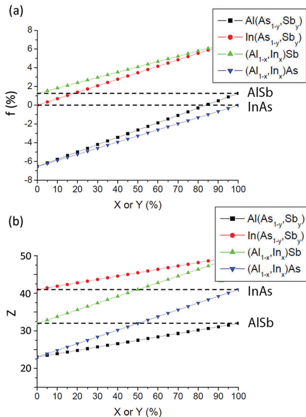
FIG. 3. (a) Misfit f with InAs and (b) average atomic number Z , for the four possible ternary compounds. The horizontal dashed lines correspond to InAs and AlSb.
