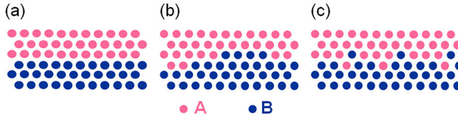
FIG. 2. Schematic representation of the different types of interface between two systems, A and B, with no common atoms. (a) Minimal interface with a simple atomic bond between A and B layers. (b) Topological interface due to roughness, generally about one atomic layer in the semiconductor materials. (c) Chemical interface where the diffusion mechanisms (for miscible materials) result in an intermediate mixed layer.
