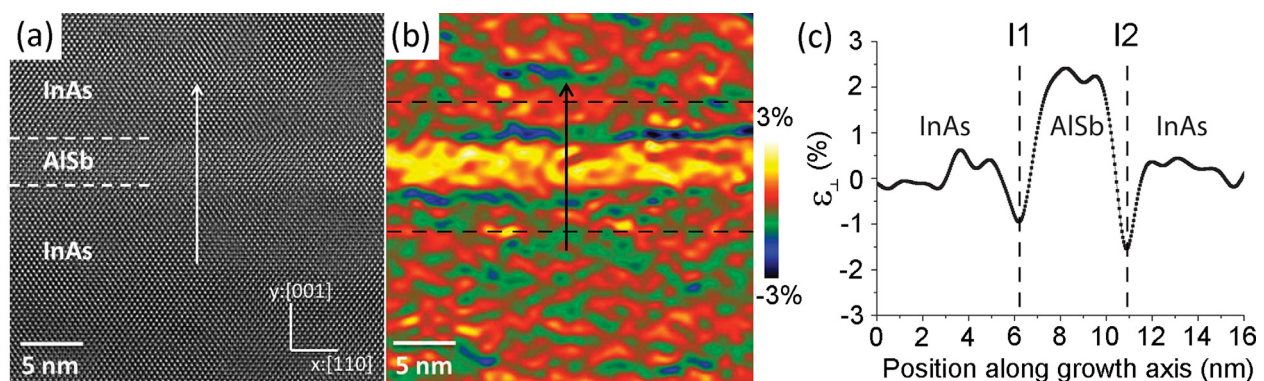
FIG. 5. (a) HRTEM image of sample A along [110] zone axis, (b) \varepsilon_{\perp} mapping, (c) \varepsilon_{\perp} strain profile obtained by GPA averaged on the whole width of the image (30 nm). The white arrow indicates the growth direction.
