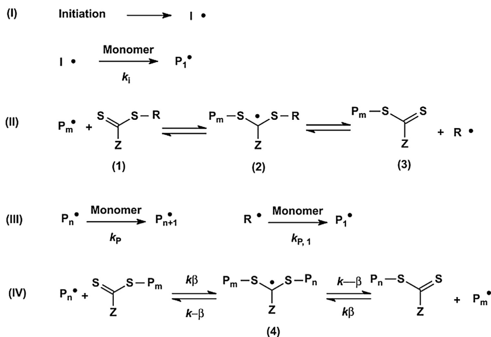
Fig. 5. Mechanism of a RAFT polymerization. The CTA plays the role of activator/deactivator. Reproduced from Ref. [86], Copyright(2002), with permission of John Wiley and Sons.
