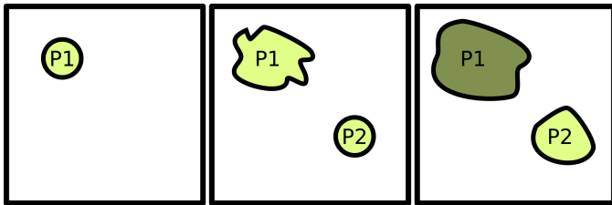
Fig. 7. From left to right: (1) a particle P1; (2) the particle P1 emits P2 and then propagates on the p-system texture’s pixels; (3) both P1 and P2 propagate, then P1 matures and its pixels change color.
