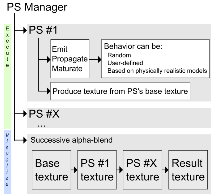
Fig. 6. Illustration of our framework (PS stands for p -system). The p -system manager goes through the p -systems, executes them and blends the textures that were produced (see examples in Fig. 13). Each p -system has an emission, a propagation and a maturation behaviors.
