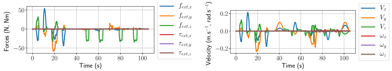
(a) Components of the external force \mathbf{f}_{ext} , applied by the human for teaching or upon collision (at t = 70 s), then by the robot during the four force control tasks.
