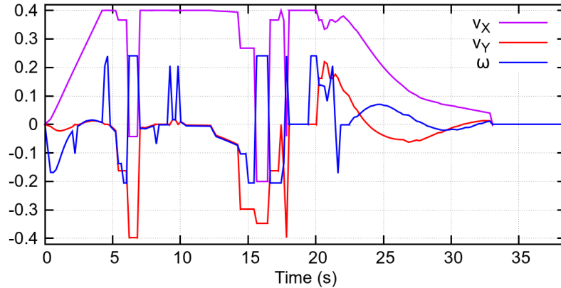
Figure 8: Real Scenario A: MPO700 Control inputs (linear velocities v_x and v_y in m/s and angular velocity \omega in rad/s).
