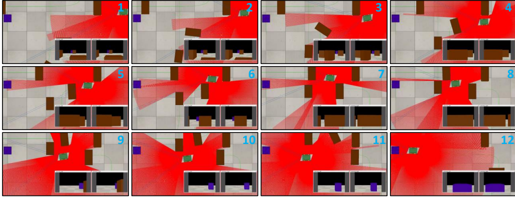
Figure 6: V-REP simulation: the robot (green box), equipped with two cameras (blue cones) and lidar scanners (red lines) navigates towards a static target (blue) while avoiding collisions and dealing with occlusions caused by one static and three moving obstacles (all brown).
