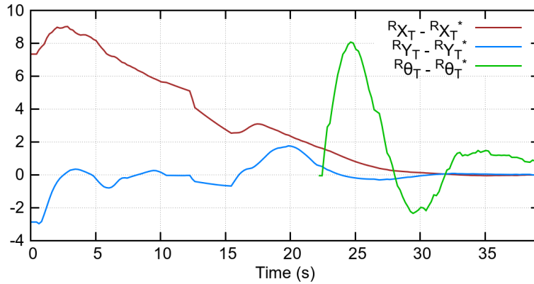
Figure 9: Real Scenario A: evolution of position (in meters) and orientation (in degrees) errors of the target in the robot frame.
