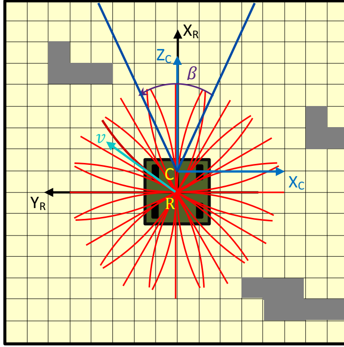
Figure 1: General definitions. The robot frame \mathcal{F}_R is shown along with the occupancy grid (yellow), occupied cells (gray), omnidirectional tentacles (red), and visual sensors center ( C ) with its field of view (blue).
