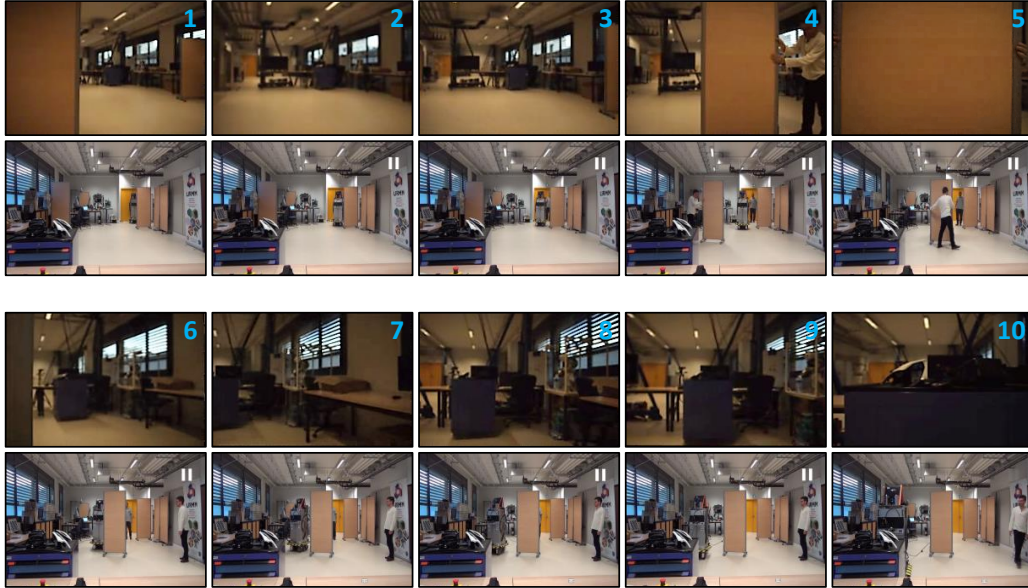
Figure 7: Real Scenario A: the MPO700 platform navigates safely towards a static blue chariot. Top: images from the left camera, bottom: the MPO700 (grey) avoids two obstacles while dealing with total target occlusion.
