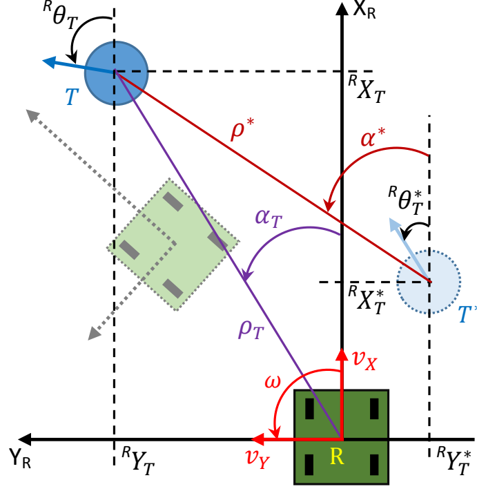
Figure 2: Definition of the visual target related variables.
