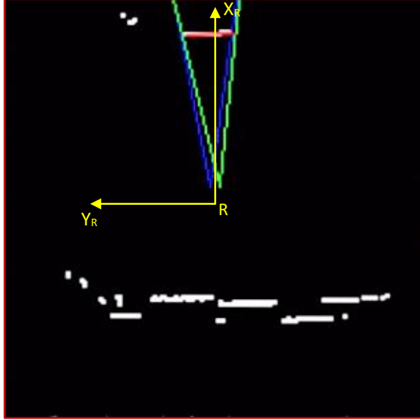
Figure 5: Detecting the cart face segment using lidar measurements.
