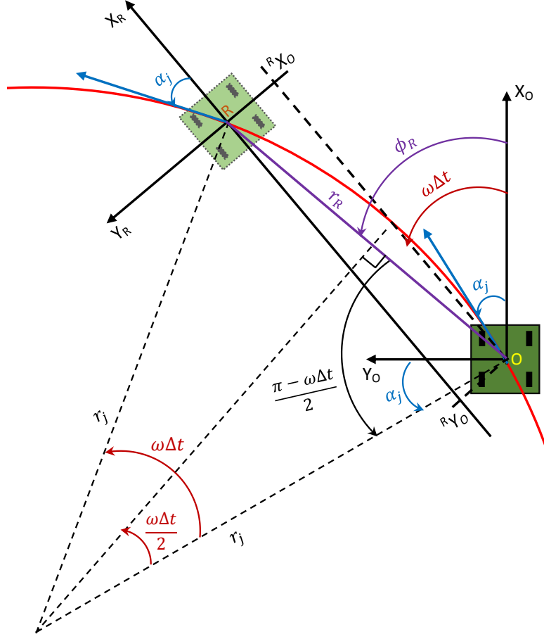
Figure 3: Variables needed for tentacle selection.
