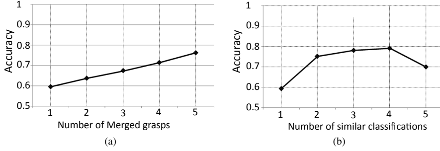
Figure 11: Recognition accuracy vs. number of combined grasps T for DF-MDAP (a) and vs. number of similar classifications k for SC-MDAP (b).
