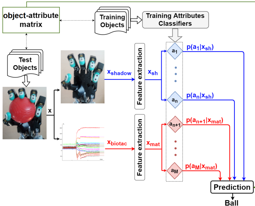
Figure 5: Our zero-shot recognition system overview.
