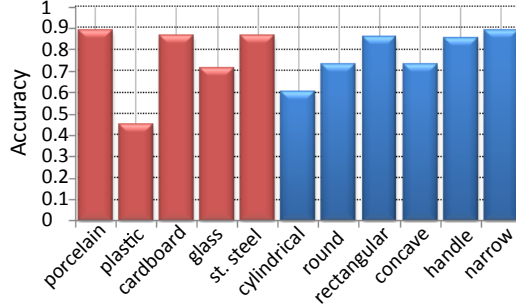
Figure 8: Recognition accuracy of attributes binary classification.
