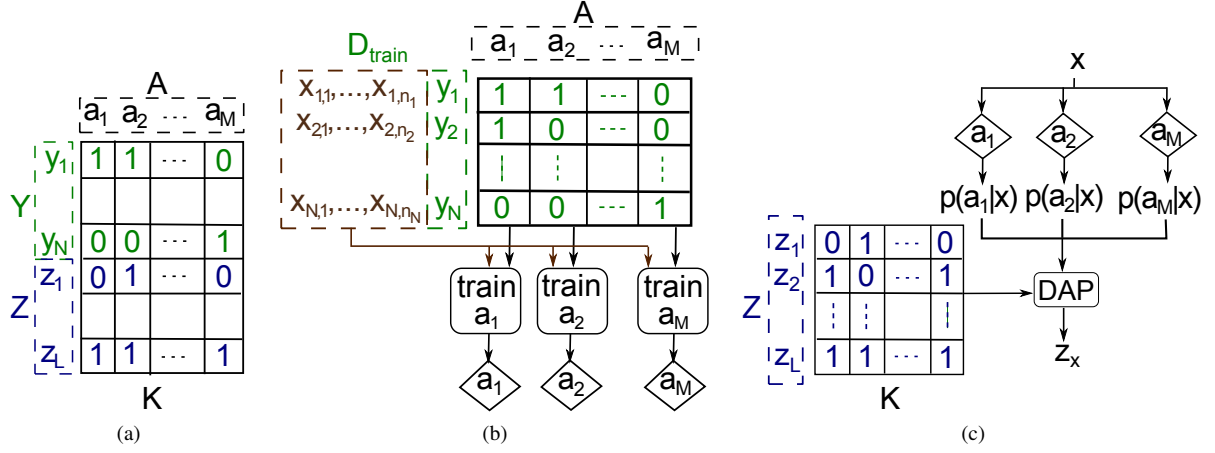
Figure 1: Attribute-based zero-shot learning: system overview.
