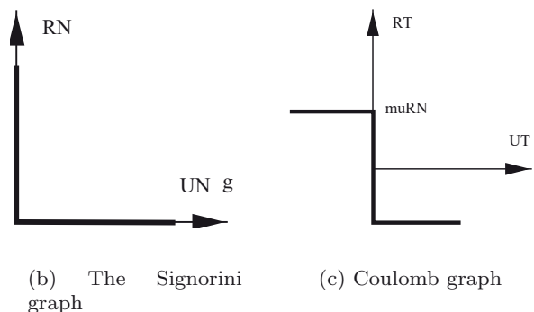
Figure 1: Contact interactions
