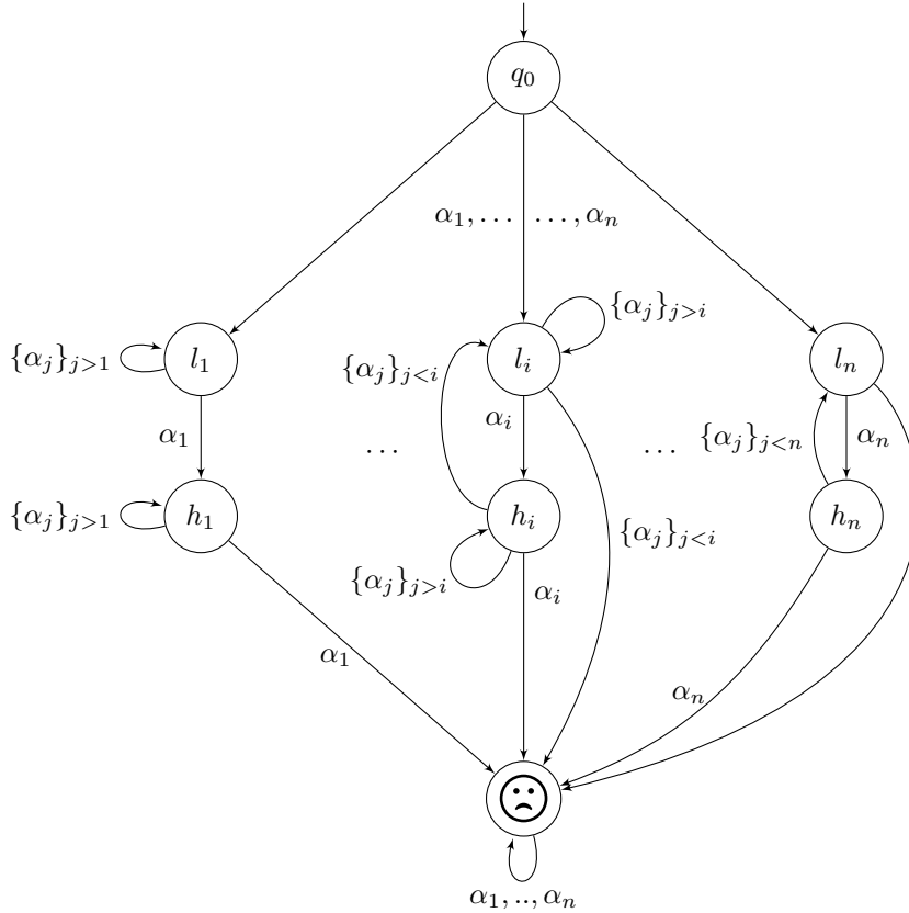
■ Figure 7 The counting gadget \mathcal{A}_{\text{count},n} .
