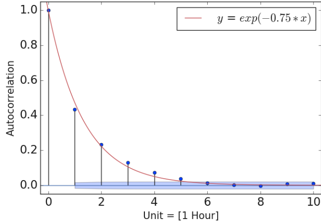
Fig. 2: Correlogram
