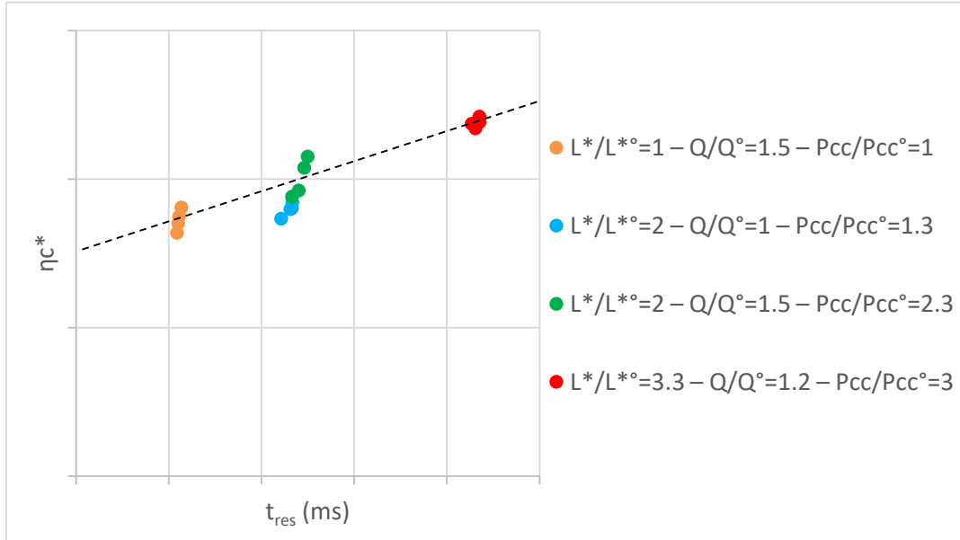
Figure 12: Evolution of the characteristic velocity efficiency versus residence time
