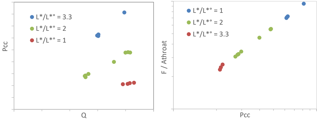
Figure 10: Evolution of combustion pressure (left), and thrust (right) in stabilized conditions
