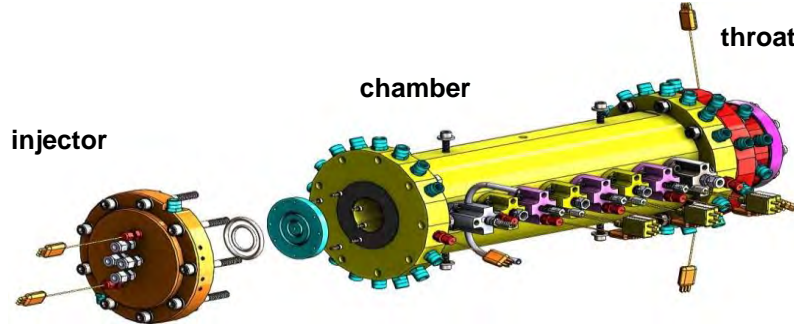
Figure 2: Mechanical assembly of the opaque combustor
