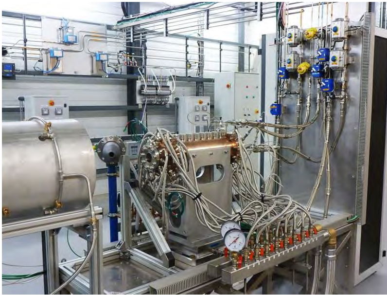
Figure 1: PERGOLA facility
