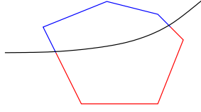
Figure 1: Hexagonal cell T cut by the interface \Gamma . The subdomain \Omega^1 (red/light grey) is located below \Gamma , and the subdomain \Omega^2 (blue/dark grey) is located above \Gamma . (\partial T)^1 is shown in red/light grey and (\partial T)^2 in blue/dark grey; the sets \mathcal{F}_{(\partial T)^1} and \mathcal{F}_{(\partial T)^2} consist each of four elements, two of which are original faces of T and two of which are sub-faces of the two faces of T cut by the interface.
