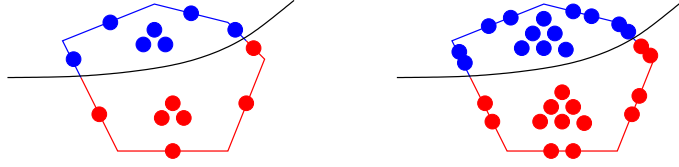
Figure 3: Cut hexagonal cell for the interface problem. The subdomain \Omega^1 (red/light grey) is located below \Gamma , and the subdomain \Omega^2 (blue/dark grey) is located above \Gamma . Left: k = 0 ; Right: k = 1 .
