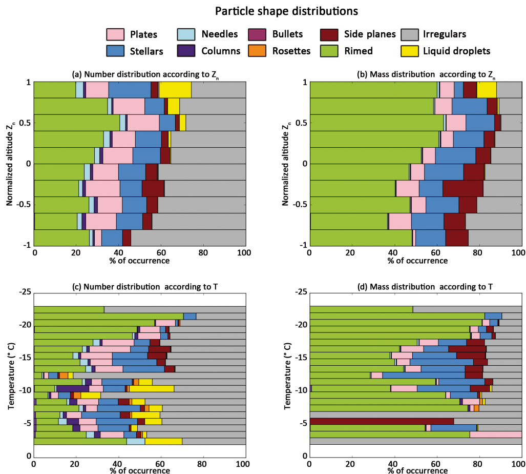
Figure 6. Vertical profiles of particle shapes (from CPI measurements and for particles larger than 100\ \mu\text{m} ) according to normalized altitude (a, b) and temperature (c, d). Distributions are displayed according to particle number (a, c) and mass (b, d).
