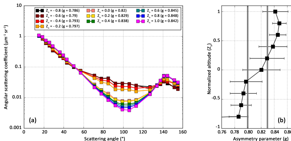
Figure 2. (a) Normalized scattering phase function according to the normalized altitude from polar nephelometer measurements (few \mu\text{m} to around 800\mu\text{m} size range), averaged over all the campaigns. g values indicate the cloud phase: g < 0.80 : ice; 0.80 < g < 0.83 : mixed; and g > 0.83 : liquid. (b) Mean vertical profile of asymmetry parameter (for all the campaigns). The grey bars indicate the threshold g values for the assessment of ice, mixed and liquid cloud phases.
