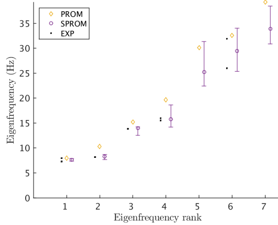
Figure 9. Real scenario of the mAEWing1 application with nonstatistical GVT data: QoIs predicted using the deterministic PROM; confidence intervals corresponding to the quantiles 0.98 and 0.02, constructed with 100 QoI samples generated by the SPROM (each circle within a confidence interval represents the statistical mean value of the corresponding QoI); averaged nonstatistical experimental values of the QoIs (EXP).
