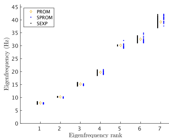
Figure 6. Hypothetical scenario for the mAEWing1 application where surrogate statistical experimental data are generated: QoIs predicted using the deterministic PROM; counterparts realized by the SPROM; counterparts realized by the random FE model (SEXP).
