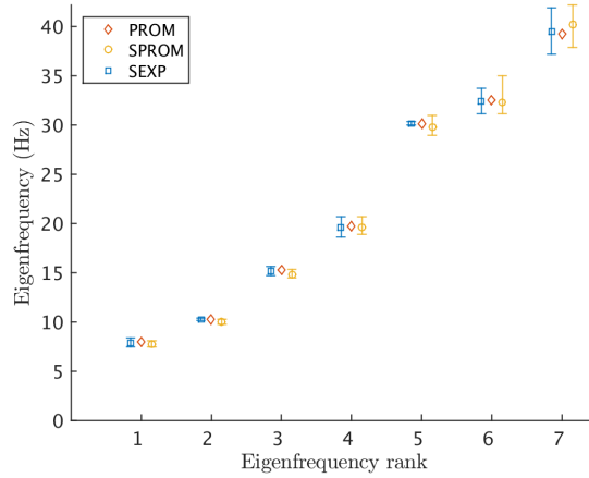
Figure 7. Hypothetical scenario for the mAEWing1 application where surrogate statistical experimental data are generated: QoIs predicted using the deterministic PROM; confidence intervals corresponding to the quantiles 0.98 and 0.02, constructed with 100 QoI samples generated by the SPROM (each circle within a confidence interval represents the statistical mean value of the corresponding QoI); counterpart confidence intervals generated by the random FE model (SEXP).
