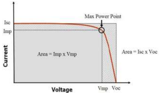
Figure 4. Fill factor
