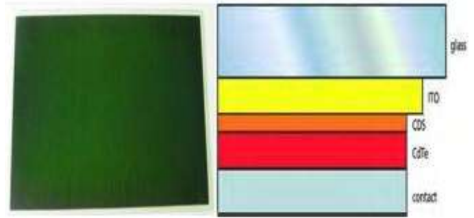
Figure 11. Cadmium telluride module and layered structure of its cell
