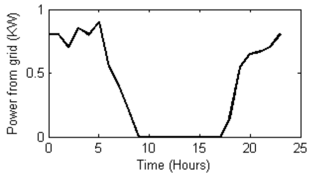
Figure 17. Power taken from the grid
