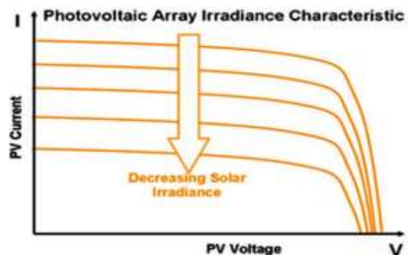
Figure 1. Effects of irradiance on current and voltage of PV module
