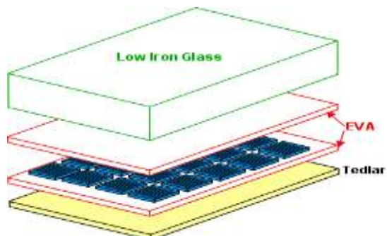
Figure 5. Layers in PV module
