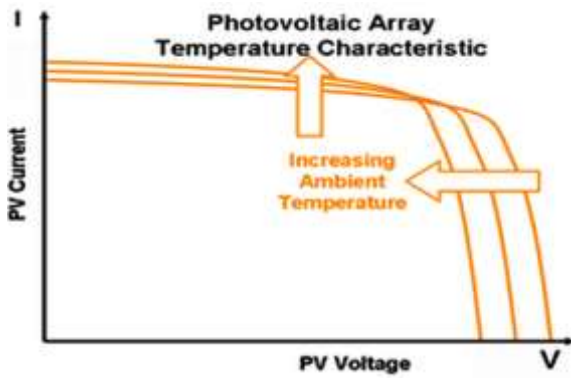
Figure 2. Effect of ambient temperature on current and voltage of module
