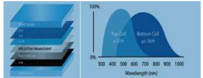
Figure 12. Layered structure of micromorphous technology with its spectrum response
