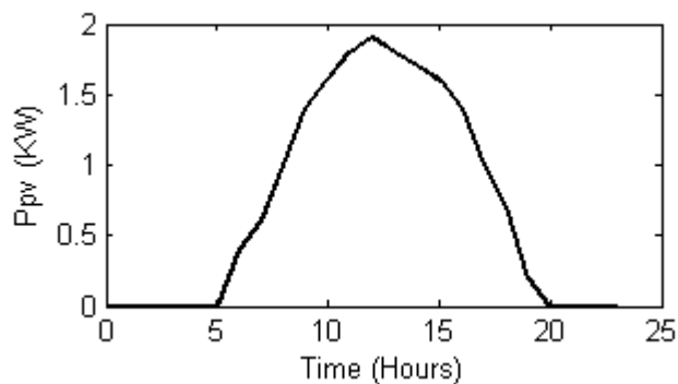
Figure 16. 2KW PV array output power
