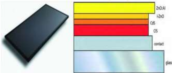
Figure 10. CIS module and CIS cell layered structure
