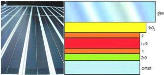
Figure 9. Amorphous modules and amorphous cell layered structure
