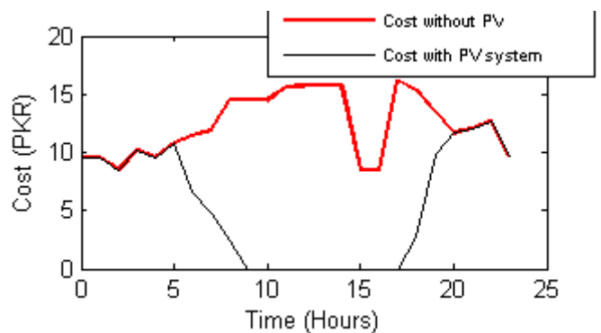
Figure 19. Cost of energy with and without PV system
