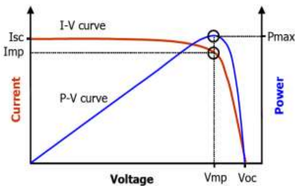
Figure 3. Maximum power point
