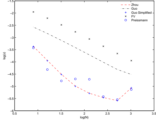
Figure 12: Precision of different methods.
