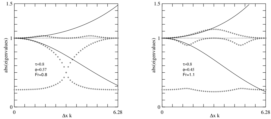
Figure 6: Norm of the eigenvalues of M_k(\tau, \phi, Fr) , as a function of k\Delta x , outside the numerical stability region. Left and right panels illustrate two different choices of \tau , \phi and Fr . The dots show the three eigenvalues obtained numerically and the lines corresponds to e^{i\omega_{\pm}\Delta t} .
