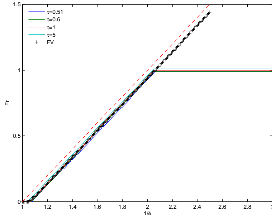
Figure 14: The stability region of LBM (lines) and finite volume method (+). The Courant condition is presented as a dashed line. There is a slight difference with Fig. 7 because the simulation is non-linear.
