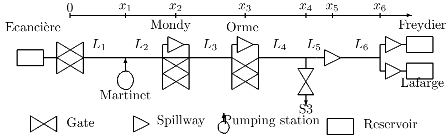
Figure 21: Structure of the Bourne irrigation system
