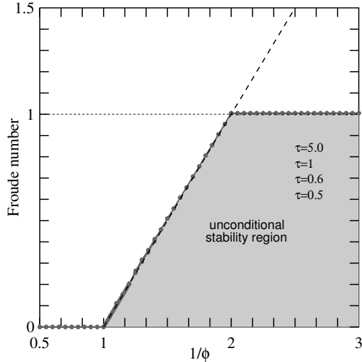
Figure 7: Stability region in the \phi^{-1} - \text{Fr} plane, for different values of \tau (gray dots), which all give the same limit. The black dashed line is the theoretical value corresponding to the Courant condition (99).
