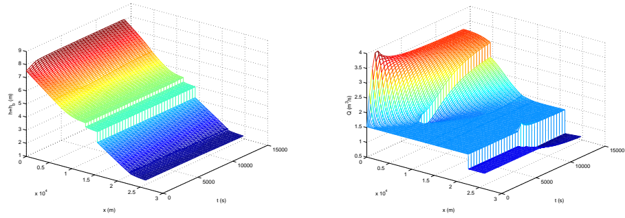
Figure 24: Evolution in the main canal
