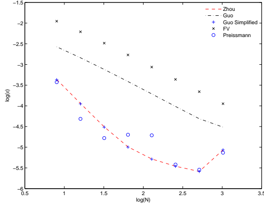
Figure 12: Precision of different methods.
