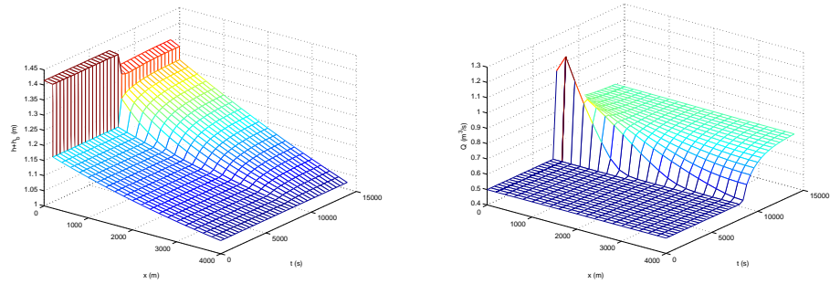
Figure 25: Evolution in the secondary canal
