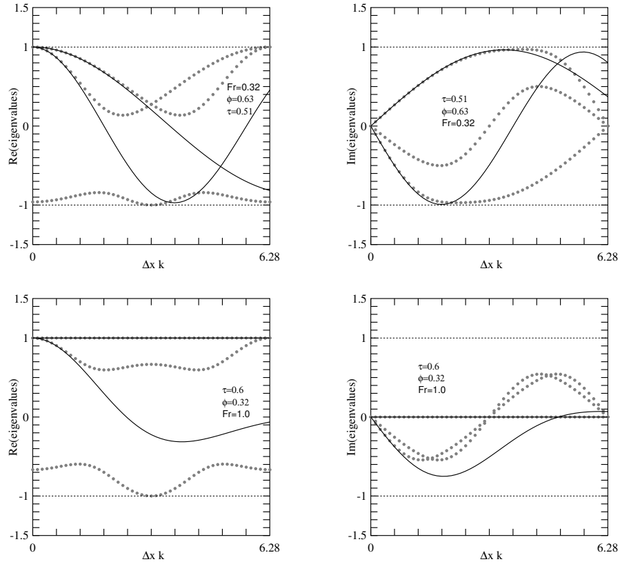
Figure 4: The real (left) and imaginary (right) parts of the eigenvalues \lambda of M_k(\tau, \phi, Fr) , as a function of k\Delta x . The eigenvalues found numerically are shown as dots and are compared to the shallow water dispersion relation e^{i\omega_{\pm}\Delta t} (solid lines). This figure illustrates two possible choices of the model parameters \tau , \phi and Fr .
