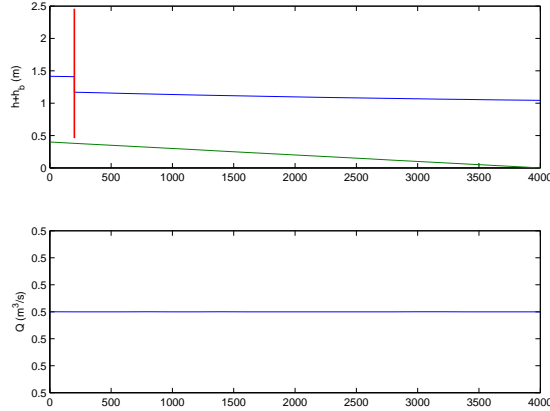
Figure 23: Initial conditions for the secondary canal
