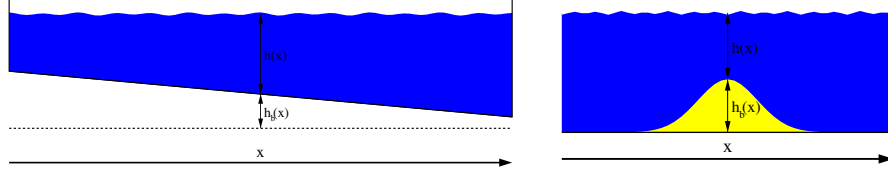
Figure 3: Two situations of a canal reach where u = 0 and h + h_b = \text{const} is an exact solution. Left: there is a net slope but two walls prevent flow motion. A computational domain with the so-called half-way bounce back left and right boundary conditions is used. Right: there is a local deformation of the bed but no global slope. A periodic computational domain can be used.
