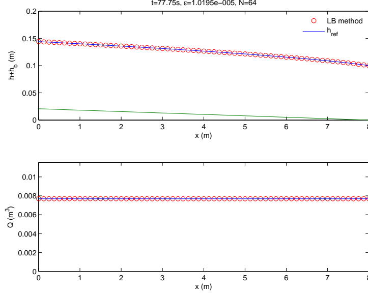
Figure 8: Steady state water level (above) and discharge (below) used for the comparison benchmark. The continuous line represents the reference solution computed from a numerical integration of the steady state shallow water equation.
