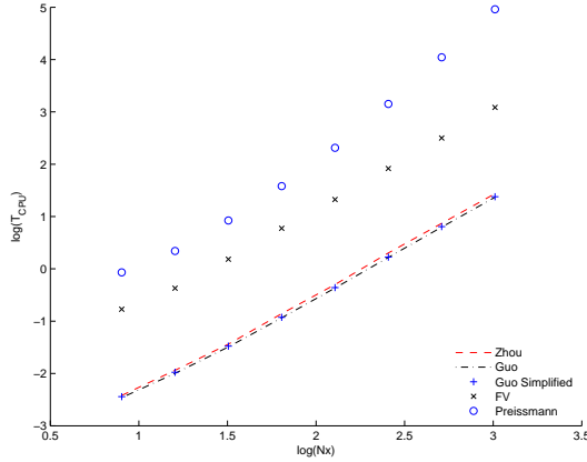
Figure 13: CPU calculation time
