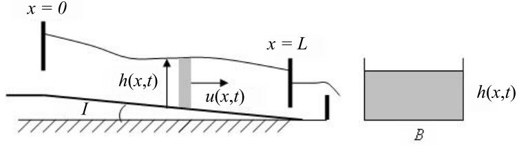
Figure 1: Longitudinal (left) and lateral (right) views of an open rectangular hydraulic channel
