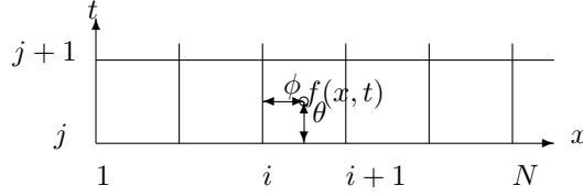
Figure 9: Preissmann implicit scheme
