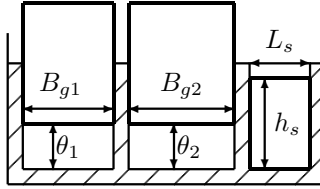
Figure 20: Structure with 2 gates and 1 spillway in parallel.
