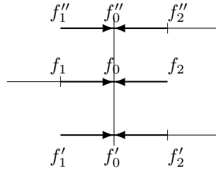
Figure 19: The known ( f'_2 , f'_0 , f''_2 , f''_0 and f_1 , f_0 ) and unknown ( f_2 , f'_1 and f''_1 ) distributions f_i at a connection point.
