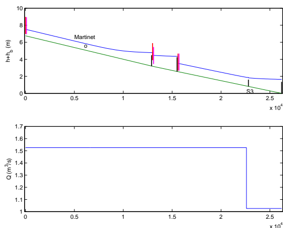
Figure 22: Initial conditions for the principal canal
