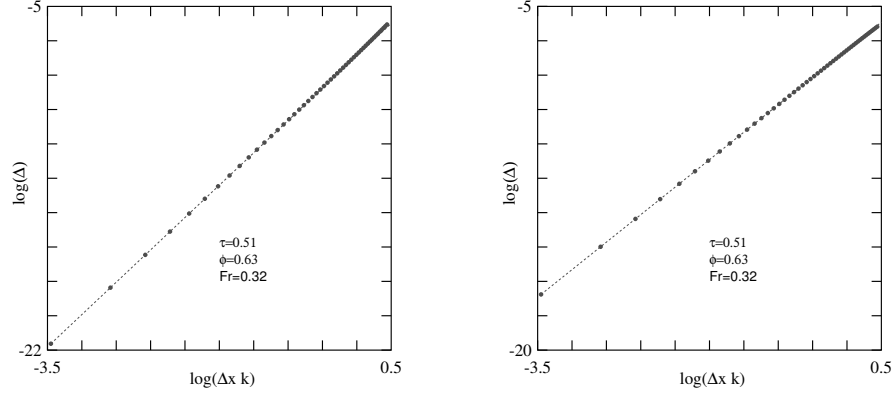
Figure 5: The dots show the value of \Delta(k\Delta x) , as given by (97) in a log-log plot. On the left, the accuracy of the real part of the dispersion relation is found to be second order because \Delta(k\Delta x) \propto k^4 , as indicated by the solid line of slope 4. On the right, we show the accuracy of the imaginary part of the dispersion relation. The error between the LB model and the shallow water equation grows as (k\Delta x)^3 , as proved by the solid line which has slope 3.
