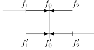
Figure 15: The known ( f'_2 , f'_0 and f_1 , f_0 ) and unknown ( f_2 and f'_1 ) distributions f_i at a connection point.
