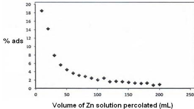
Fig. 1. Plot of the % of zinc adsorbed as a function of the volume of zinc solution percolated.
