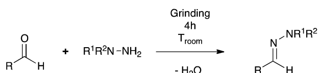
Scheme 1 General synthesis of hydrazones in the solid-state by co-grinding of a hydrazine and an aldehyde.
