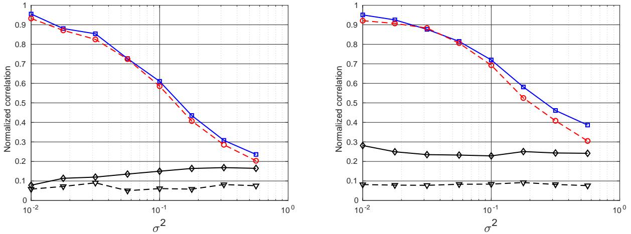
Fig. 2: Evolution of the (averaged) normalized correlation as a function of the variance \sigma^2 for K = 2 (left) and K = 5 (right), Comparison of the performance of conventional (delay-and-sum) beamforming (triangle mark), “prSAMP” (diamond mark), “paVBEM” (circle mark) and “paSAMP” with EM noise learning (square mark). Experiments show that “paSAMP” provides better results and successfully integrates the phase noisy observation model.
