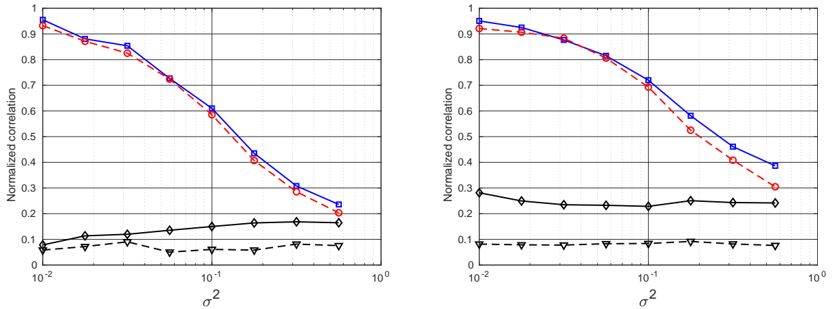
Fig. 1: Evolution of the (averaged) normalized correlation as a function of the variance \sigma^2 for K = 2 (left) and K = 5 (right), Comparison of the performance of conventional (delay-and-sum) beamforming (triangle mark), “prSAMP” (diamond mark), “paVBEM” (circle mark) and “paSAMP” (square mark). Experiments show that “paSAMP” provides better results and successfully integrates the phase noisy observation model.
